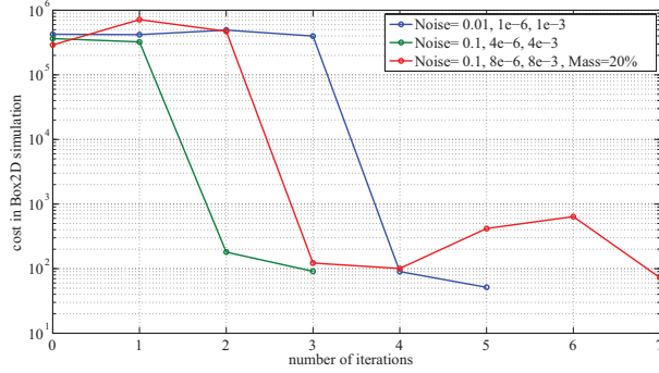
Figure 43: Change of cost function value in Box2D simulations over iterations.
