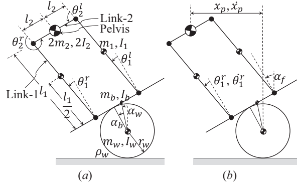
Figure 40: Robot balancing on a bongoboard.
