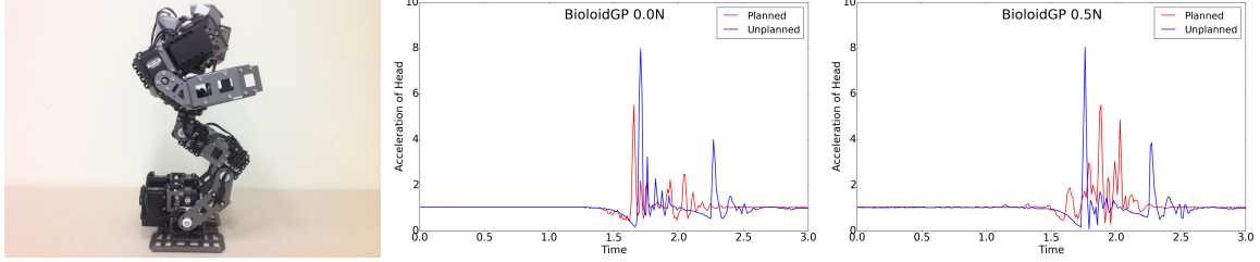
Figure 24: We measured the acceleration at the head of BioloidGP (Left). For both 0.0N (Middle) and 0.5N (Right) cases, the planned motions (Red) yielded about 68% of the maximum acceleration of the unplanned motions (Blue).
