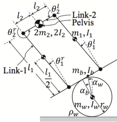
Figure 4: A design of a simple legged robot on a bongboard.
