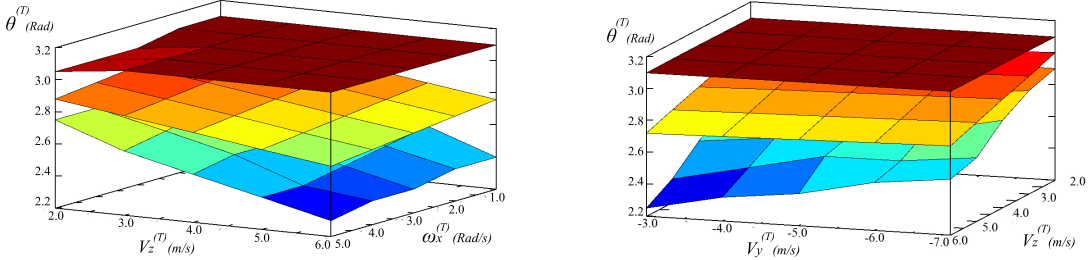
Figure 11: Samples for hands-first landing strategy. Successful samples are bounded between top and bottom planes along \theta^{(T)} axis. The middle plane, average of the two, indicates the linear relation of the ideal landing condition.
