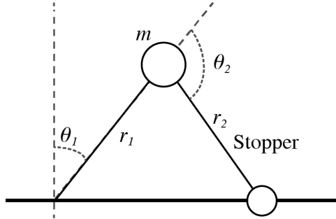
Figure 20: The abstract model consists of a telescopic inverted pendulum and a massless stopper.
