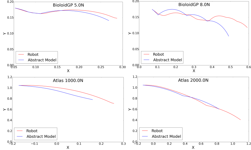
Figure 23: COM trajectories between the abstract model (Blue) and the robot (Red). Top left: BioloidGP forward falling from a one-foot stance due to a 5.0N push. Top right: BioloidGP forward falling from a one-foot stance due to a 8.0N push. Bottom left: Atlas forward falling from a two-foot stance due to a 1000N push. Bottom right: Atlas forward falling from a two-foot stance due to a 2000N push.
