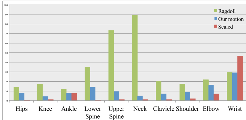
Figure 18: Maximal stress for each joint from a hands-first landing motion. Results are quantitatively similar across all of our simulations. Green: Ragdoll motion. Blue: Our motion. Orange: Joint stress scaled by mass.
