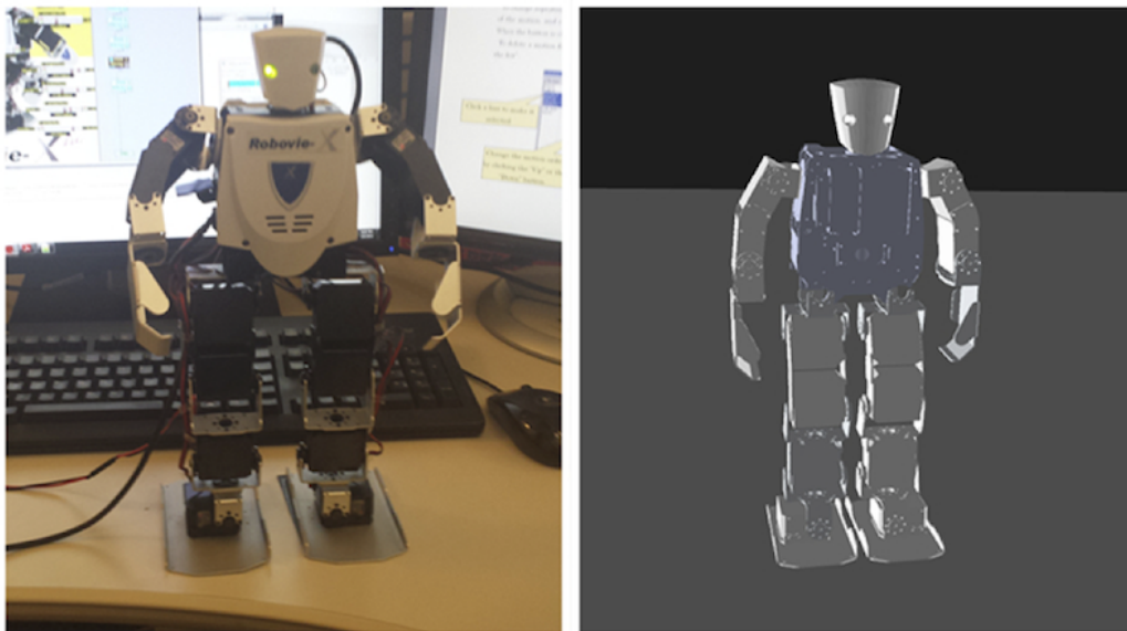
Figure 6: Difference between a real robot and its simulation model results different motions from same controllers.
