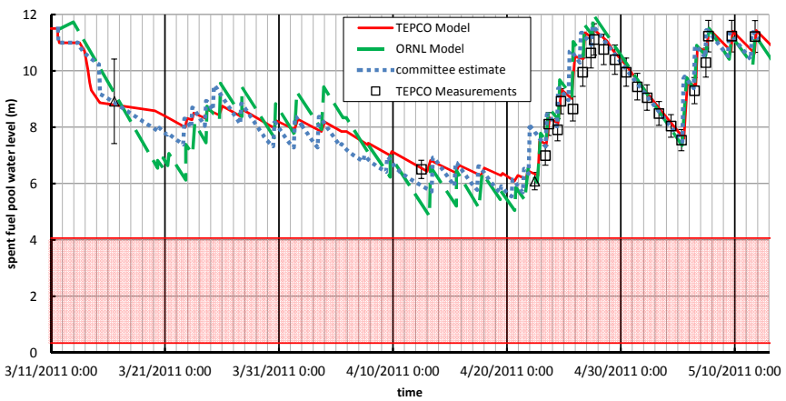
FIGURE 2.16 Comparison of Unit 4 spent fuel pool water-level estimates from TEPCO (2012a) (red curve), ORNL (Wang et al., 2012) (green curve), and the present committee (dotted blue curve). Note: Also shown are the measurements of pool water levels made by TEPCO starting on April 22 (black squares).
