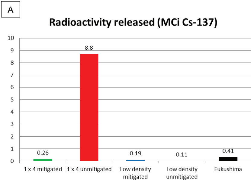
FIGURE 7.3 Selected consequences from the Spent Fuel Pool Study as a function of fuel loading (1 × 4 loading; low-density loading) and mitigation required by 10 CFR 50.54(hh)(2). Notes: Consequences for the Fukushima Daiichi accident are shown for comparison. (A) Radioactive material releases. (B) Land interdiction (see footnote 26 for an explanation of the values for the Fukushima bar). (C) Displaced populations. SOURCE: Table 7.1 in this report; IAEA (2015), NRA (2013), NRC (2014, Chapter 6), UNSCEAR (2013).
