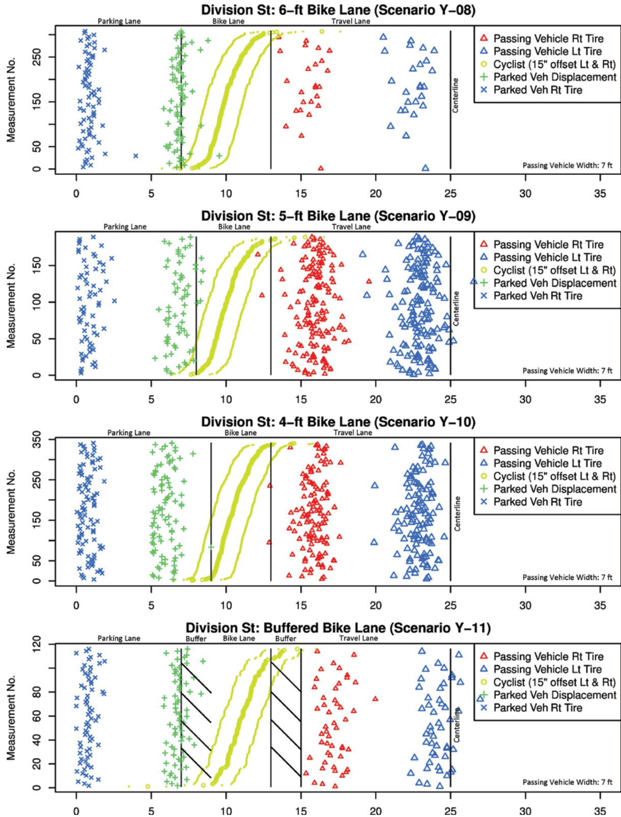
Figure 11. Measurements taken on Division Street in Chicago (assumed 7-ft width for passing vehicle).
