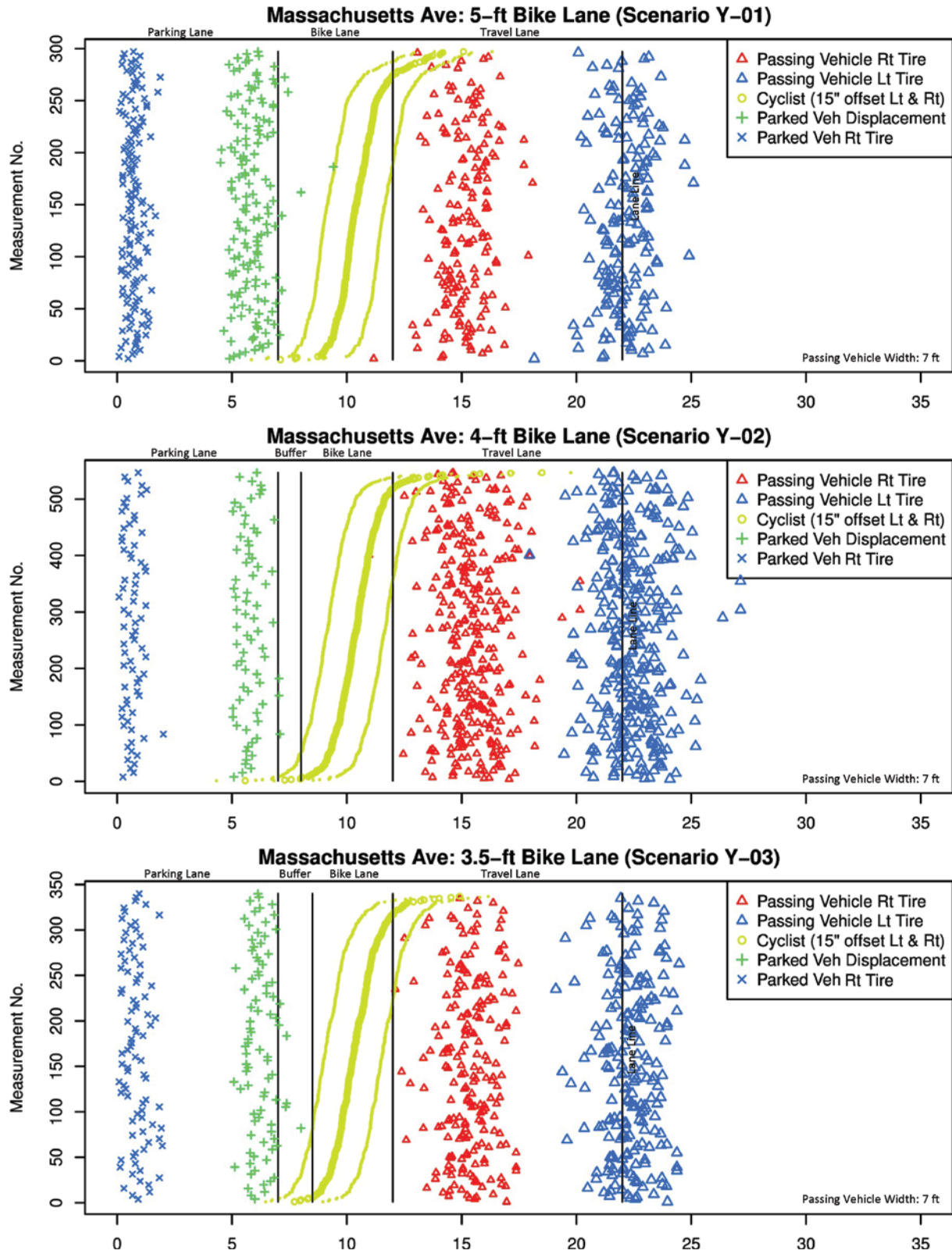
Figure 9. Measurements taken on Massachusetts Avenue in Cambridge (assumed 7-ft width for passing vehicle).
