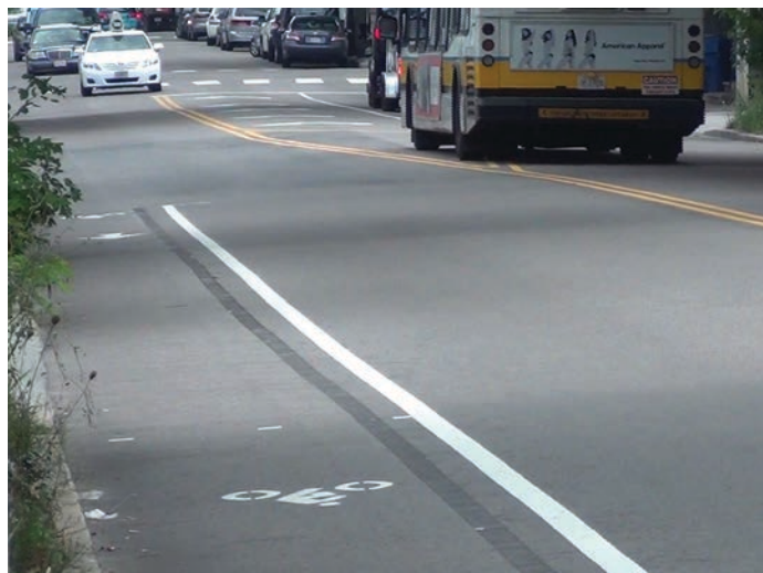
5-ft Bike Lane (Scenario N-4)
