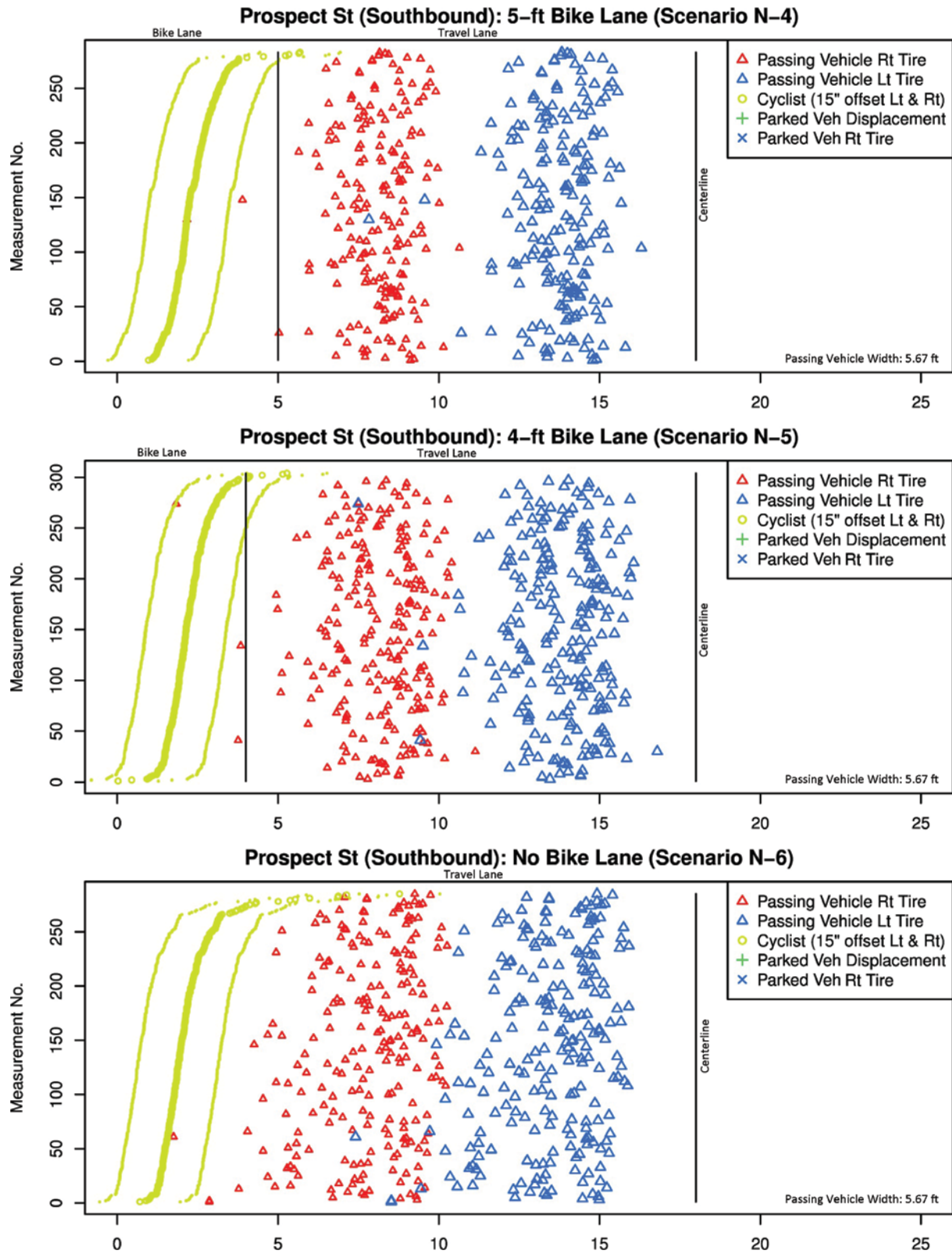
Figure 18. Measurements taken on Prospect Street (southbound) in Cambridge (assumed 5.67-ft width for passing vehicle).
