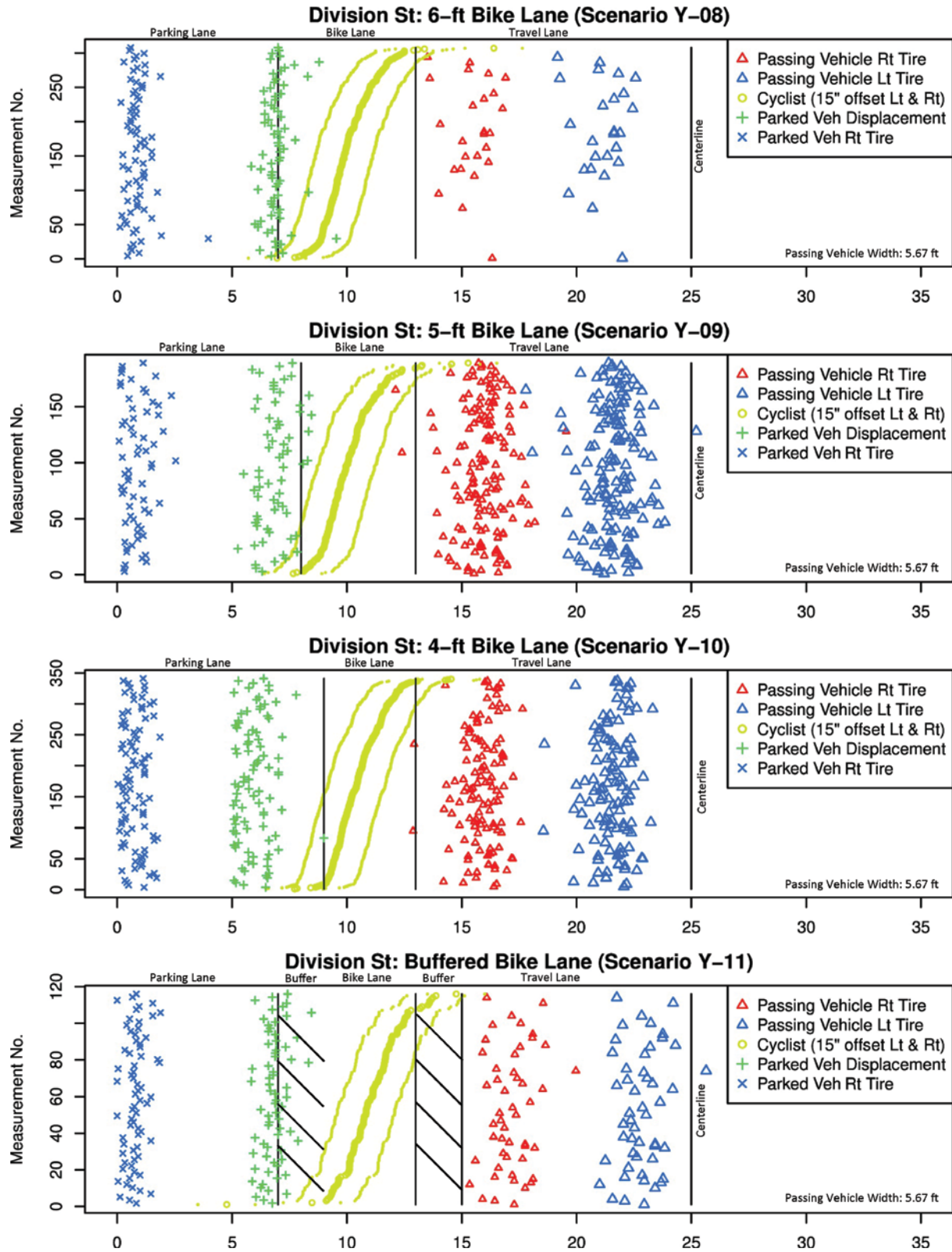
Figure 16. Measurements taken on Division Street in Chicago (assumed 5.67-ft width for passing vehicle).
