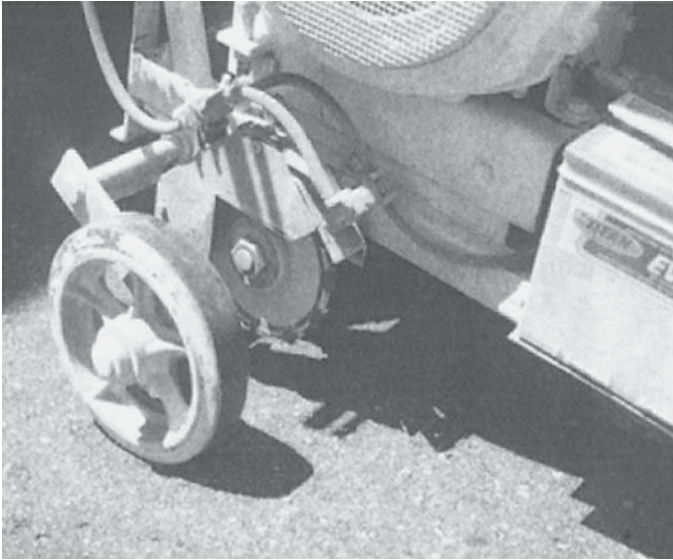
Photographs 4-4. Diamond saw crack cutting (16).
