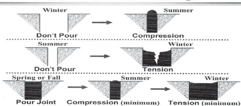
Graphic 4-5. Not the right time for crack treatment (SS-1).
