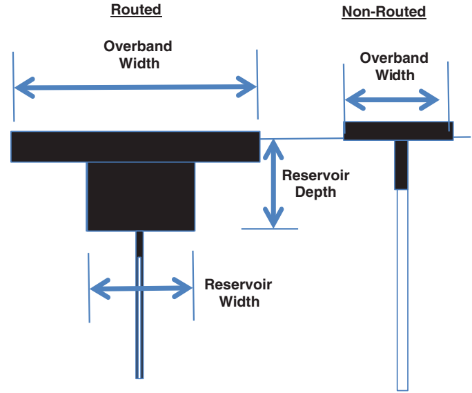
Graphic 3-3. Overband crack treatment configuration, both routed (left) and non-routed (right).
