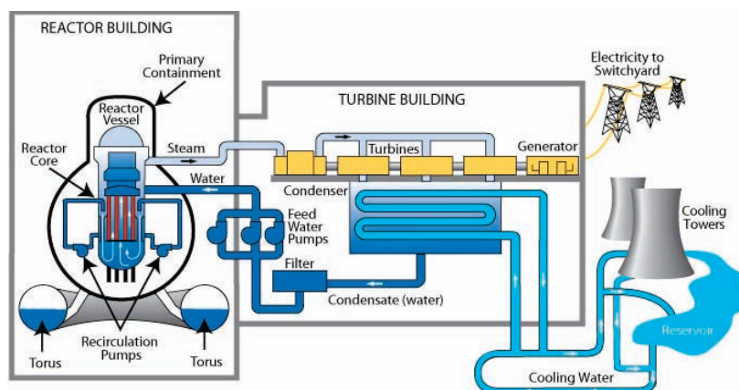
FIGURE 2.16 In a boiling water reactor system the reactor core generates heat which is absorbed by pure water that is moved through the core to produce a steam-water mixture. The steam is separated from the water and directed to the turbine to turn the turbine generator to produce electricity. Unused steam is condensed to water and pumped back to the reactor. As with the pressurized light-water reactor system, the reactor core is cooled by water circulated by electrical pumps. SOURCE: EIA (2012f).
