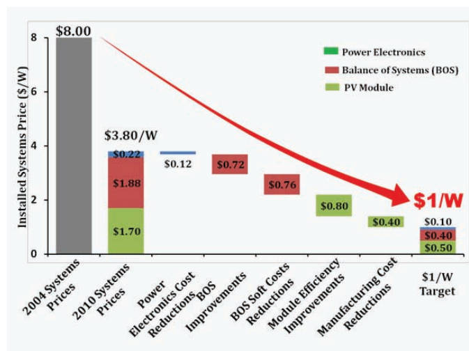
FIGURE 3.4 Price reductions to achieve the SunShot Initiative goal of $1/watt PV system costs. SOURCE: Friedman (2011).
