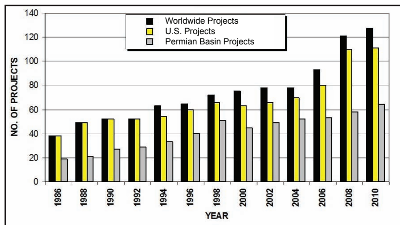
FIGURE 3.18 Number of projects using CO 2 -EOR: worldwide, United States and the Permian Basin, West Texas. SOURCE: Melzer (2012, p. 4).
