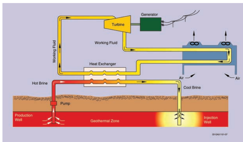
FIGURE 3.14 A binary power plant using an air-cooled condenser. When wet cooling is used, a cooling tower similar to one in a flash plant replaces the air cooler, requiring a source of water because all of the geothermal fluid is injected back into the reservoir. SOURCE: Courtesy of Idaho National Laboratory.
