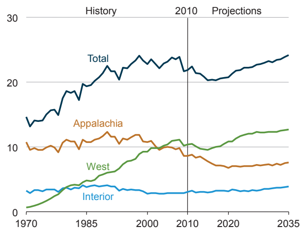
FIGURE 2.26 Coal production by region, 1970-2035, Reference case (quadrillion Btu). SOURCE: EIA (2012a, Fig. 118, p. 98).
