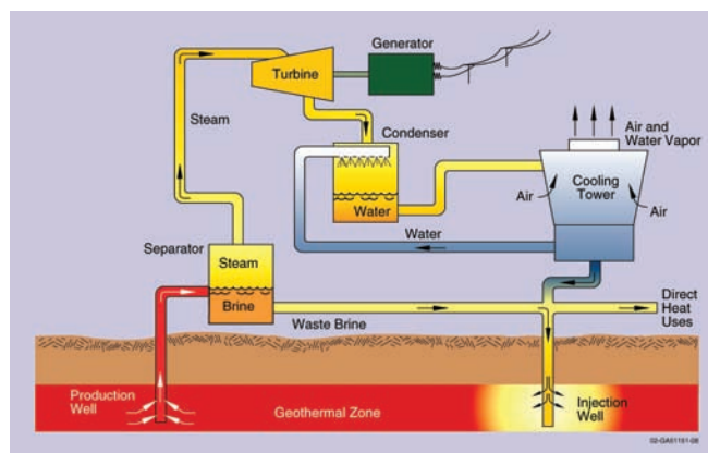
FIGURE 3.13 A flashed-steam power plant. SOURCE: Courtesy of Idaho National Laboratory.
