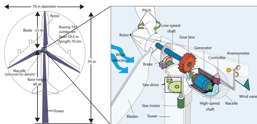
FIGURE 3.5 Typical 1.5-MW-class wind turbine system. SOURCE: Wilburn, (2011, Fig. 1, p. 2).
