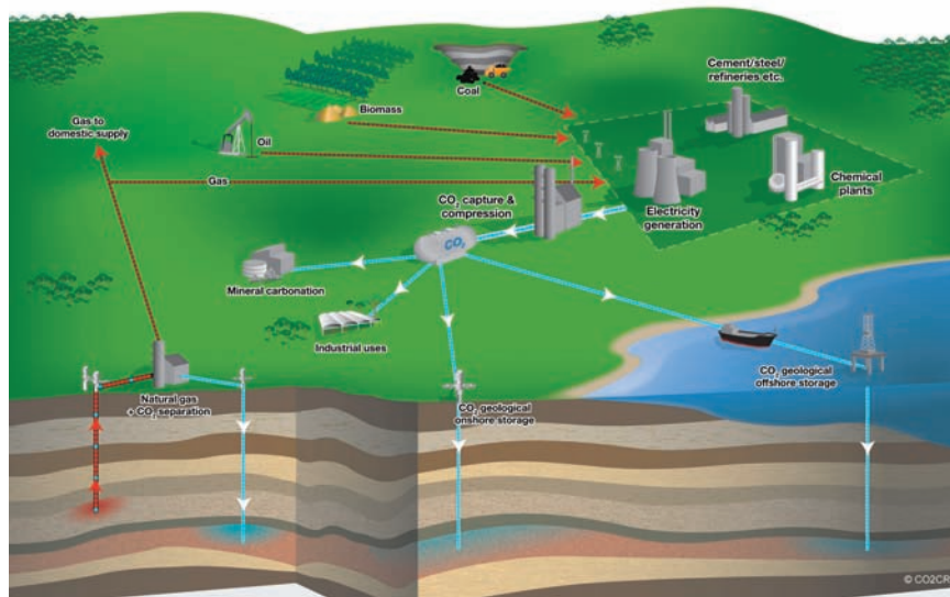
FIGURE 3.17 Schematic of the carbon dioxide capture and sequestration process. SOURCE: Reprinted with permission from CO2CRC.
