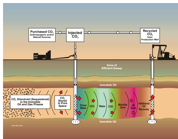
FIGURE 3.21 Schematic showing the processes of CO 2 -EOR. SOURCE: ARI/Melzer (2010, Fig. 1, p. 3).
