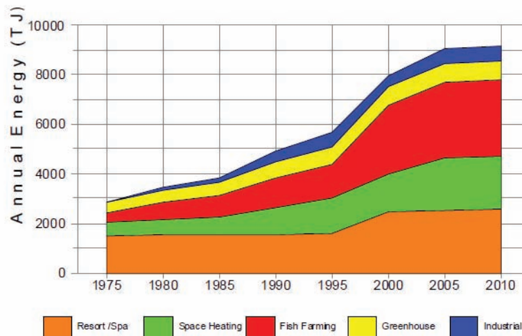
FIGURE 3.16 Direct-use growth in the United States without heat pumps. SOURCE: Tony Boyd, Geo-Heat Center.
