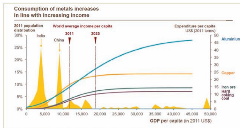
FIGURE 2.25 Consumption of major metals and coking coal increases in concert with increasing income. Also shown is the percent of global population with respect to per capita income. The U.S. population is the yellow peak at the extreme right of the diagram. SOURCE: Rio Tinto (2012, p. 40). Used with permission from Rio Tinto.
