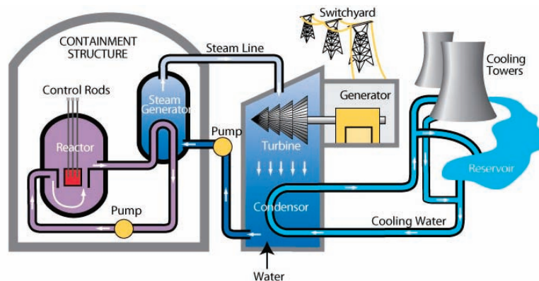
FIGURE 2.15 In a pressurized light-water reactor system, the reactor core produces heat which is carried by the pressurized water in a coolant loop to the steam generator. This heat in the steam generator, in turn, vaporizes the water in a secondary loop into steam which turns the turbine generator to produce electricity. Unused steam is condensed into water, which is pumped back to the steam generator. The reactor core is cooled by water circulated by electrical pumps. SOURCE: EIA (2012g).
