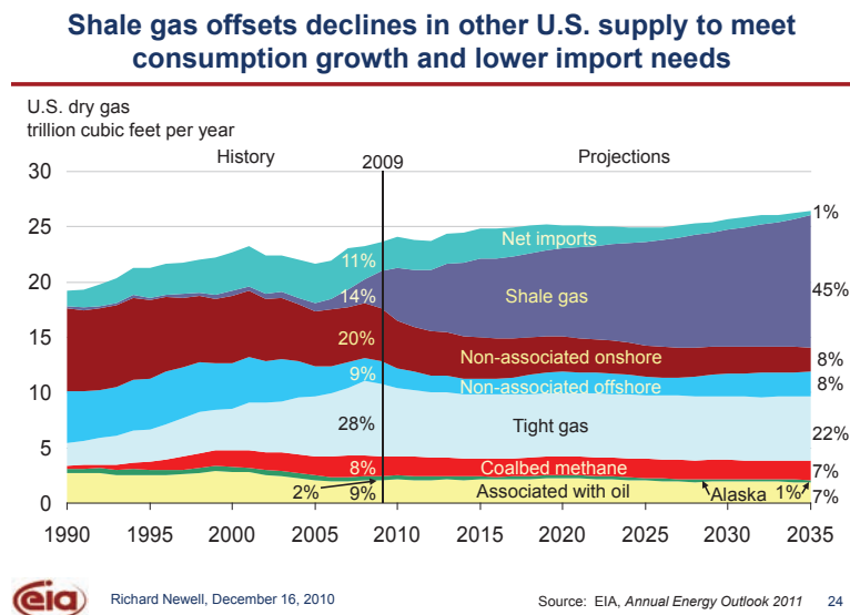
FIGURE 2.2 EIA historical and future production trends for gas by reservoir type. SOURCE: Newell (2010).
