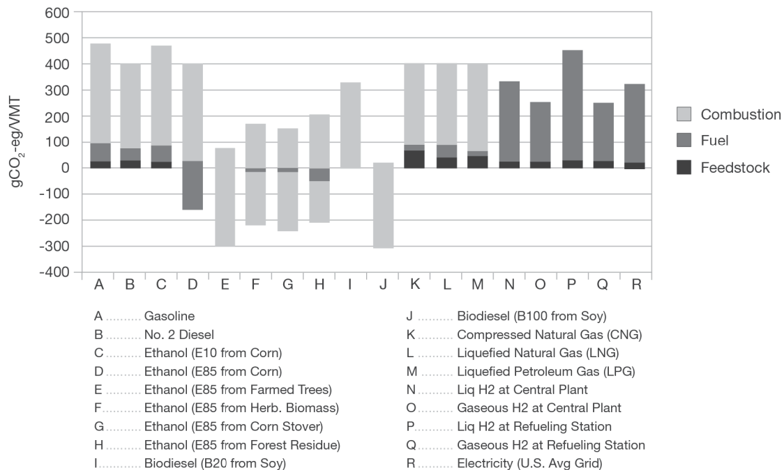
Figure 2.9. Relative GHG emissions from different fuels using GREET model.
