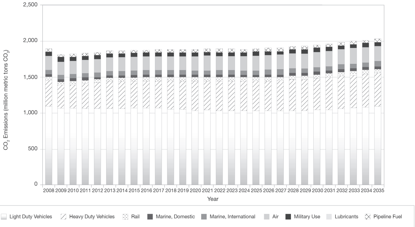
Figure 2.4. Future inventory of transportation-related GHG emissions by mode.
