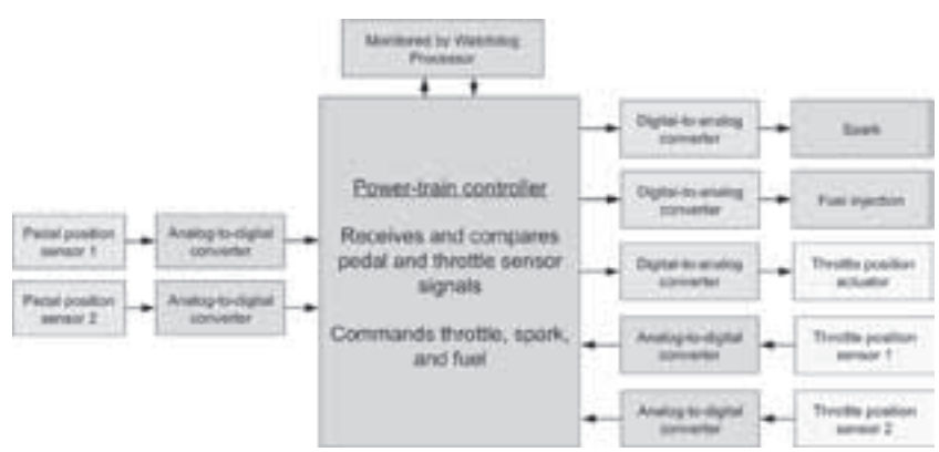
FIGURE 3-1 ETC input and output flows.
