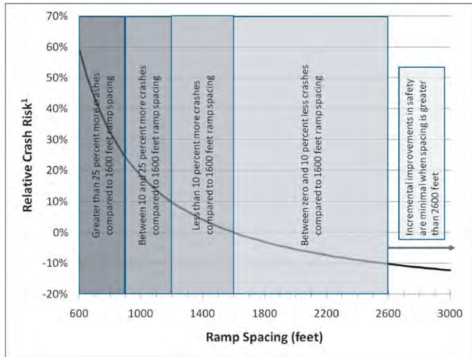
1 Relative crash risk is measured by the percent difference in crashes, of all types and severities, at some ramp spacing value compared to a ramp spacing of 1,600 ft
