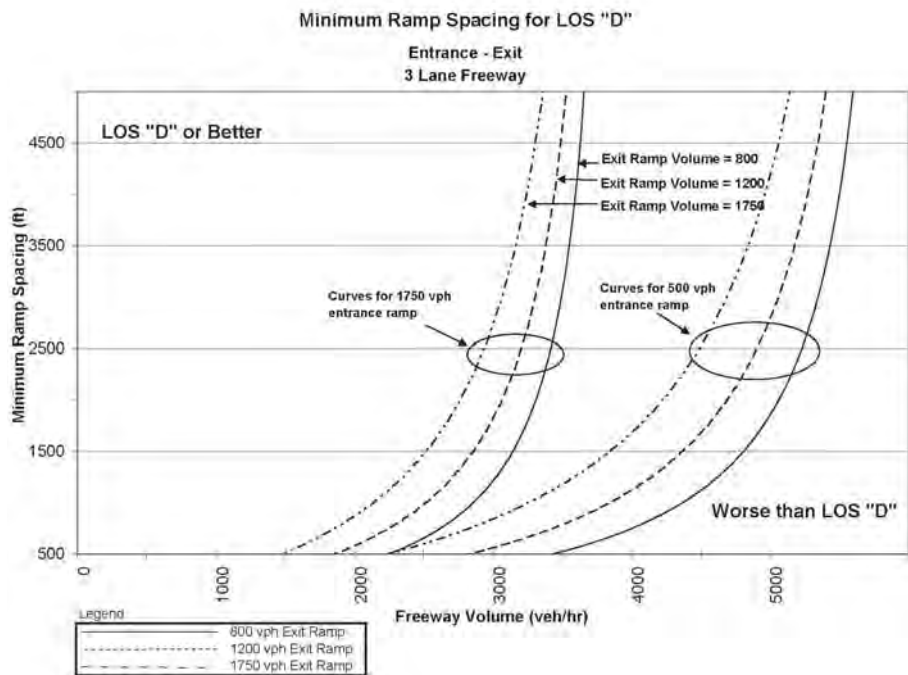
Minimum Ramp Spacing to Achieve LOS D on a Three-Lane Freeway
