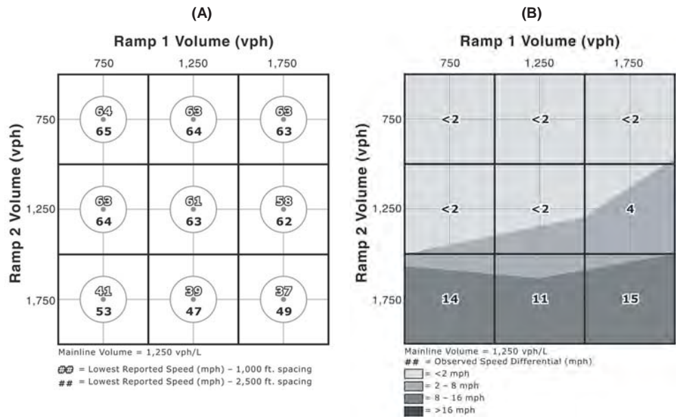
Entry-Exit Mainline Entering Volume 1,250 vph/L, 1,000-ft spacing and 2,500-ft spacing:
