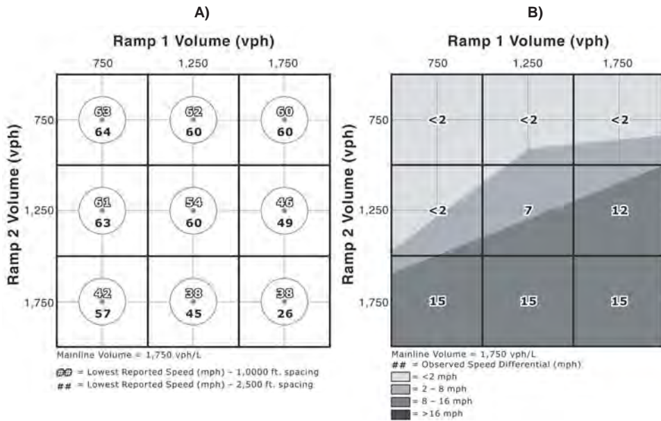
Entry-Exit Mainline Entering Volume 1,750 vph/L, 1,000-ft spacing and 2,500-ft spacing: A) Comparison of Lowest Speed Reported, B) Maximum Corresponding Point-Speed Difference
