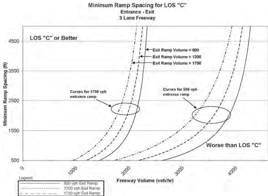
Minimum Ramp Spacing to Achieve LOS C on a Three-Lane Freeway
