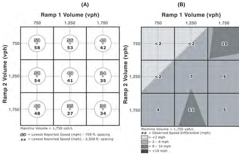
Entry-Entry Mainline Entering Volume 1,750 vph/L, 700-ft spacing and 2,500-ft spacing: (A) Comparison of Lowest Speed Reported, (B) Maximum Corresponding Point-Speed Difference
