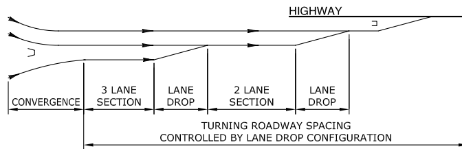
Exhibit 3-5 Effect of Lane Drops on a Turning Roadway
