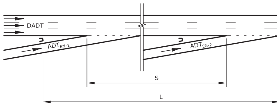
Exhibit 5-9 Key Variables for Planning and Preliminary Design Safety Assessment: Entrance Ramp followed by Entrance Ramp
