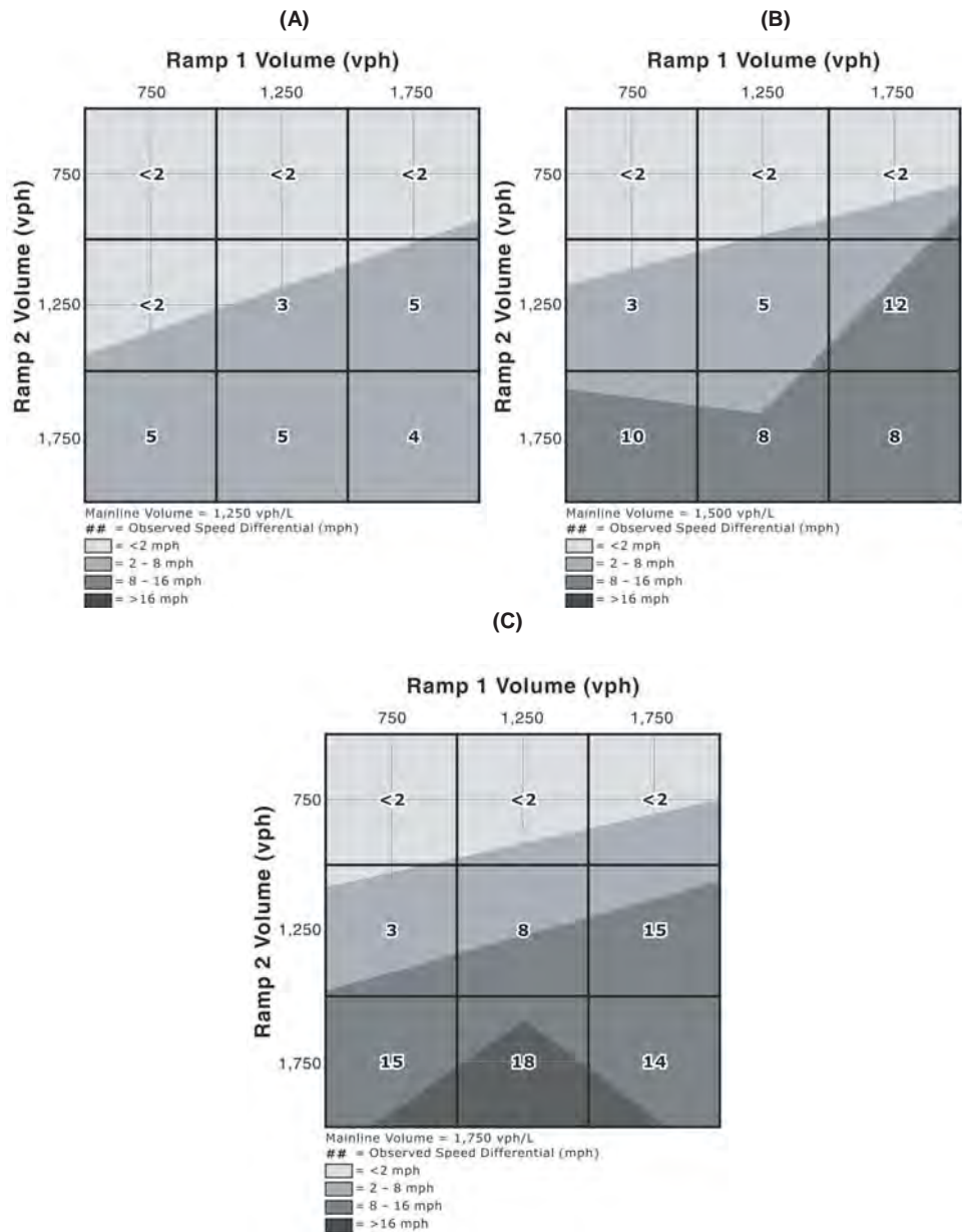
Effect of Auxiliary Lane on Mainline Speed (1,000-ft ramp spacing)
