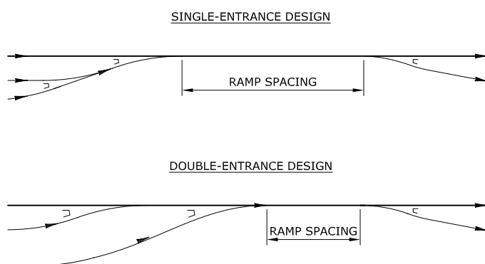
Exhibit 3-1 Single and Multiple Entrance Ramps
