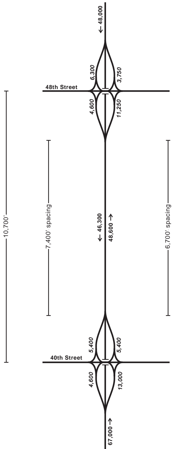
CASE STUDY 3 RAMP SPACING AND DAILY TRAFFIC VOLUMES WITHOUT 44TH STREET INTERCHANGE
