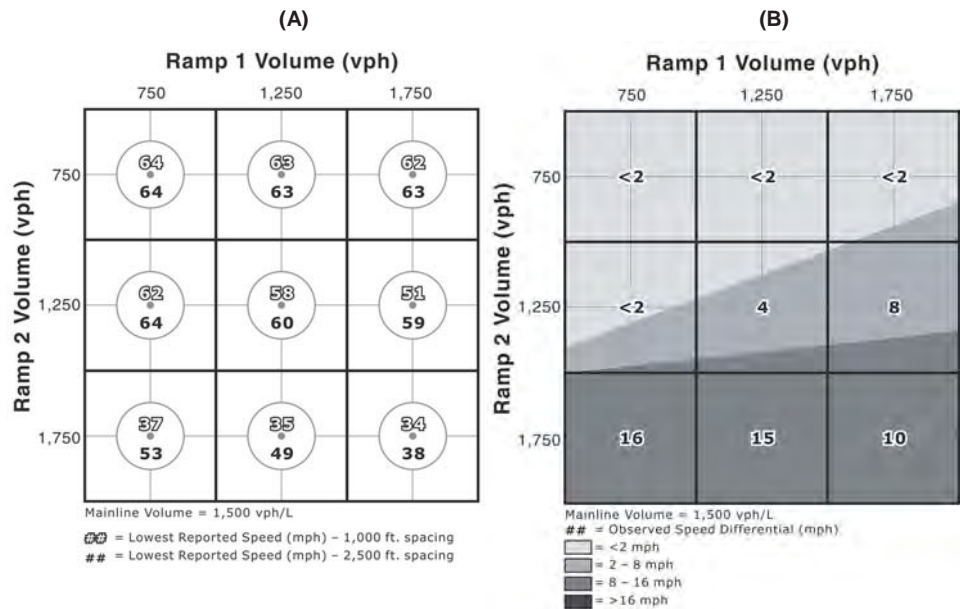
Entry-Exit Mainline Entering Volume 1,500 vph/L, 1,000-ft spacing and 2,500-ft spacing:
