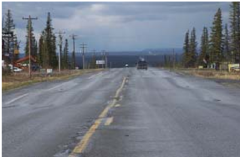
Typical permafrost damage on the Glenn Highway near Glennallen, Alaska.
