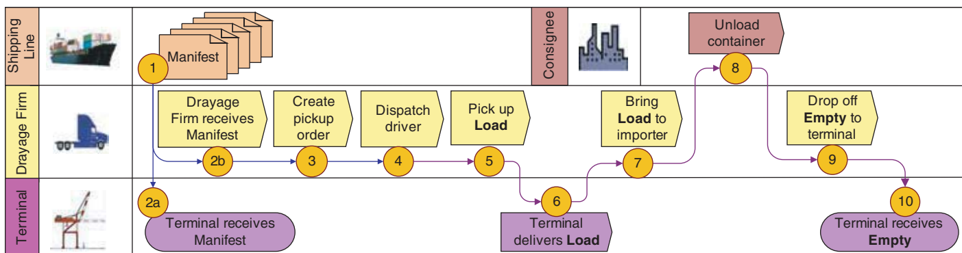
Figure 2–3. Import drayage process map.
