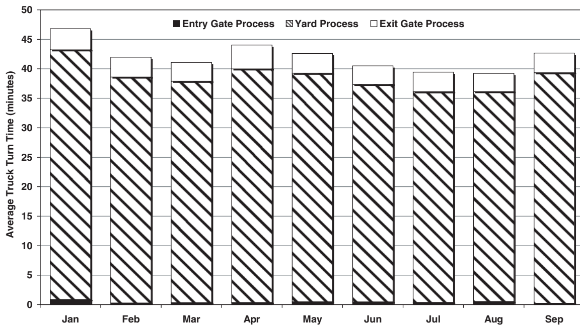
Figure 5-3. Drayage turn time segments.
