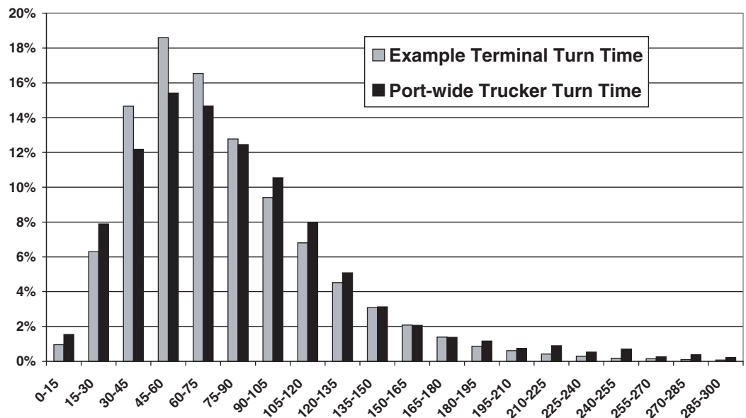
Figure 5-2. Trucker and terminal turn time comparison.
