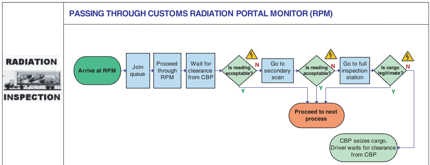
Figure 2–9. RPM subprocesses.
