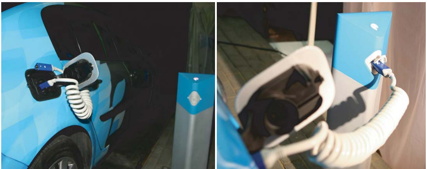
Figure 34. Charging electric car—designed by Better Place.
