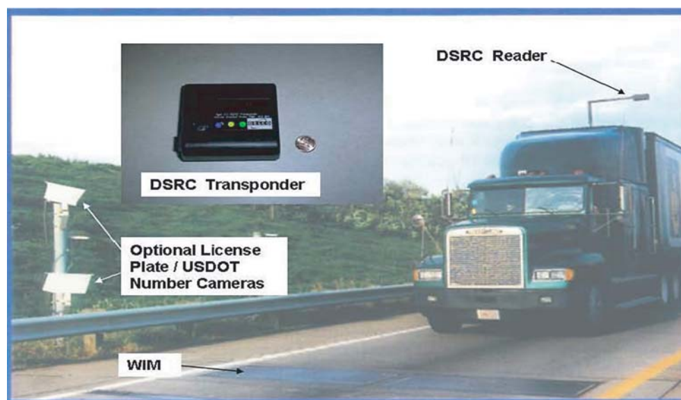
Figure 31. Example of electronic screening equipment.
