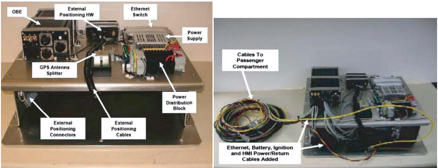
Figure 18. OBE with other external parts (left) and cables (right).
