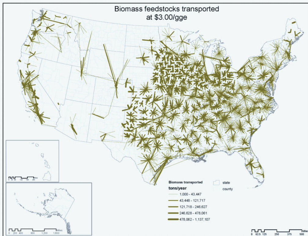
FIGURE 3-4 Biomass deliveries to the biorefineries needed to meet the RFS2 consumption mandate in 2022 projected by the National Biorefinery Siting Model.
