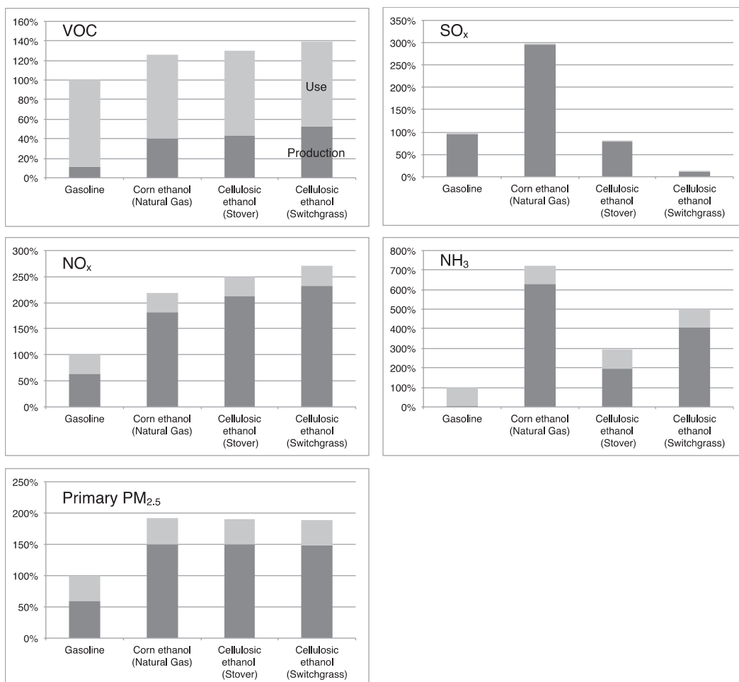
FIGURE 5-4 Life-cycle emissions of volatile organic compounds (VOCs), sulfur oxides (SO x ), nitrous oxides (NO x ), ammonia (NH 3 ), and primary particulate matter 2.5 (PM 2.5 ) from gasoline, dry-mill corn-grain ethanol produced using natural gas at the biorefinery, cellulosic ethanol from corn stover, and cellulosic ethanol from switchgrass.
