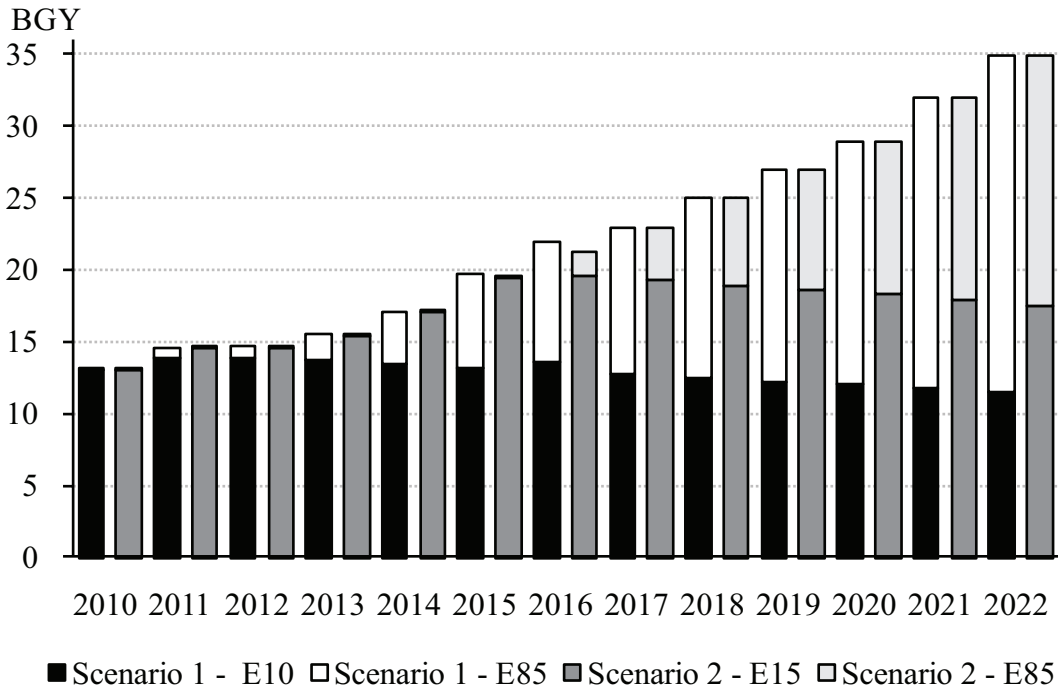
FIGURE N-2 Projected consumption of E10 and E85 under scenario 1 in which the ethanol can be used as E85 blend in FFVs or E10 in conventional vehicles, and under scenario 2 in which ethanol can be used as E85 blend in FFVs or E15 in conventional vehicles.
