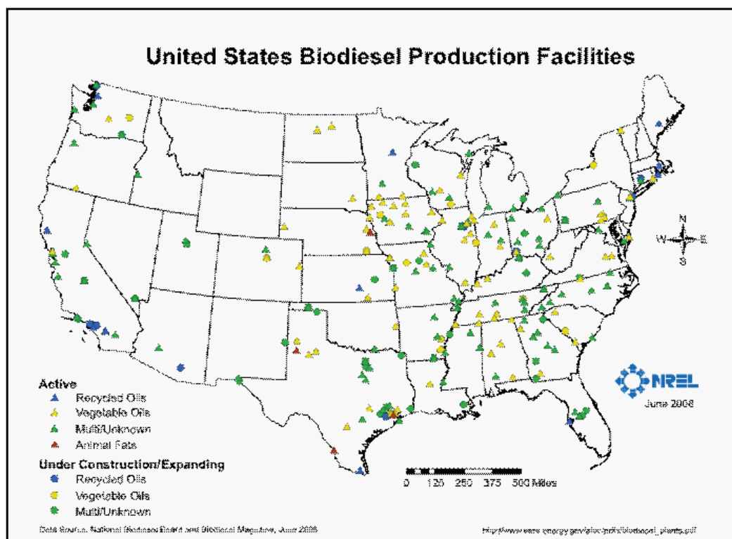
FIGURE 2-8 Biodiesel refineries in the United States (2008).
