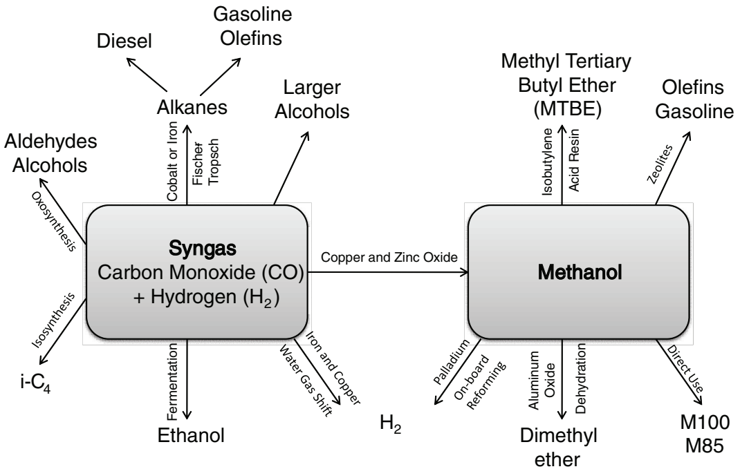
FIGURE 2-15 Thermochemical conversion pathways and products. SOURCE: Adapted from Spath and Dayton (2003).
