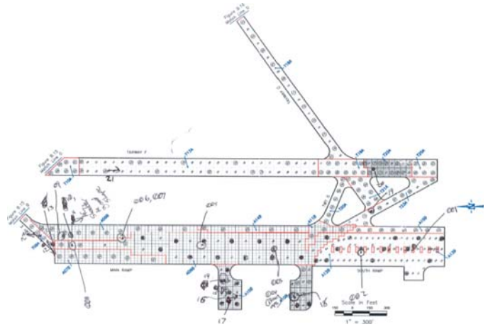
Figure 2.10. Example data recorded by dead reckoning.
