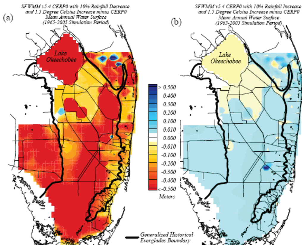
FIGURE 6-5 Simulation results using the South Florida Water Management Model showing average annual water surface elevation difference for the CERP project with modified rainfall and evapotranspiration: (a) -10 percent precipitation and +1.5°C and (b) +10 percent precipitation and +1.5°C, minus the CERP project base run (i.e., no change in precipitation and temperature).
