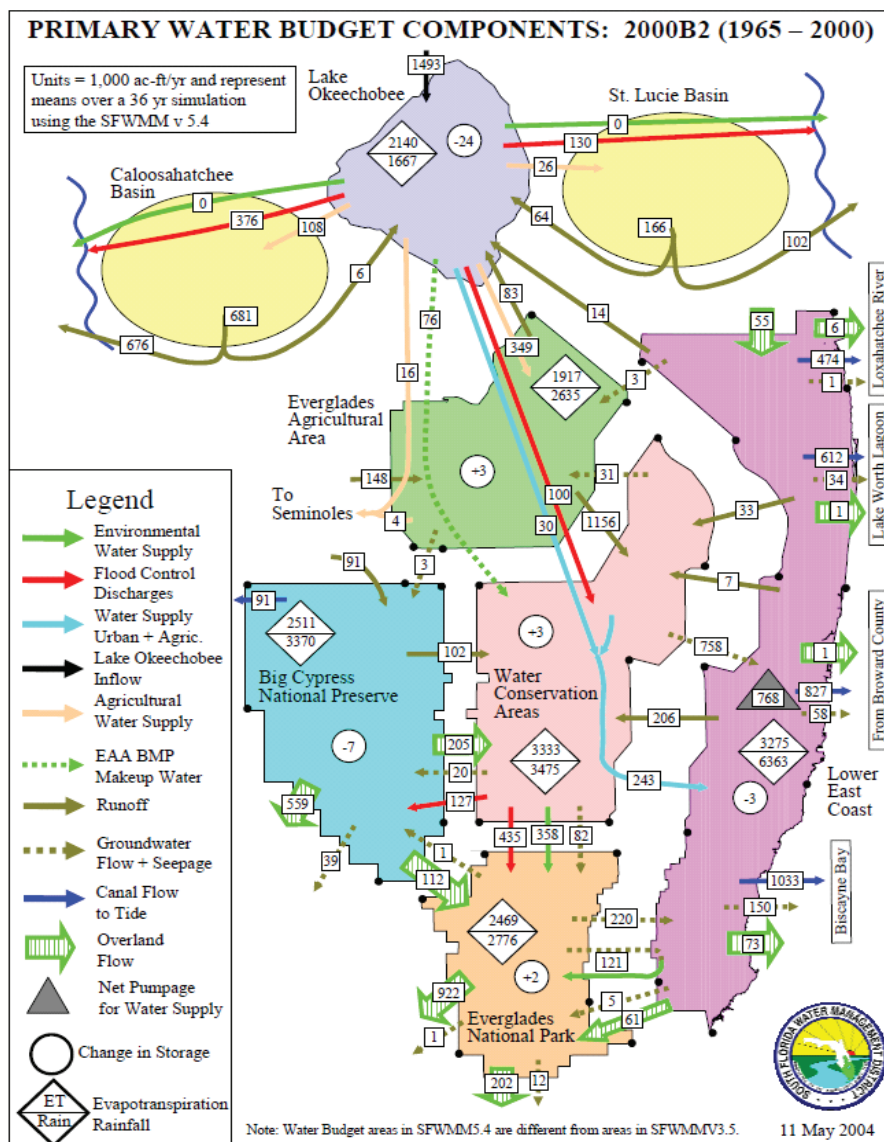
FIGURE 4-2 Estimated annual water budget for the Kissimmee-Okeechobee-Everglades drainage basin under post-drainage and post-development conditions, calculated using a 36-year simulation using the SFWMM with structures in place as of 2000 (usually considered the typical “current” situation). The numbers in rectangles represent mean annual flow volumes in 1,000 acre-feet/year, based on model simulations using a 36-year precipitation data set. Change in storage, shown in circles, represents the net inflows minus outflows over the period of record.
