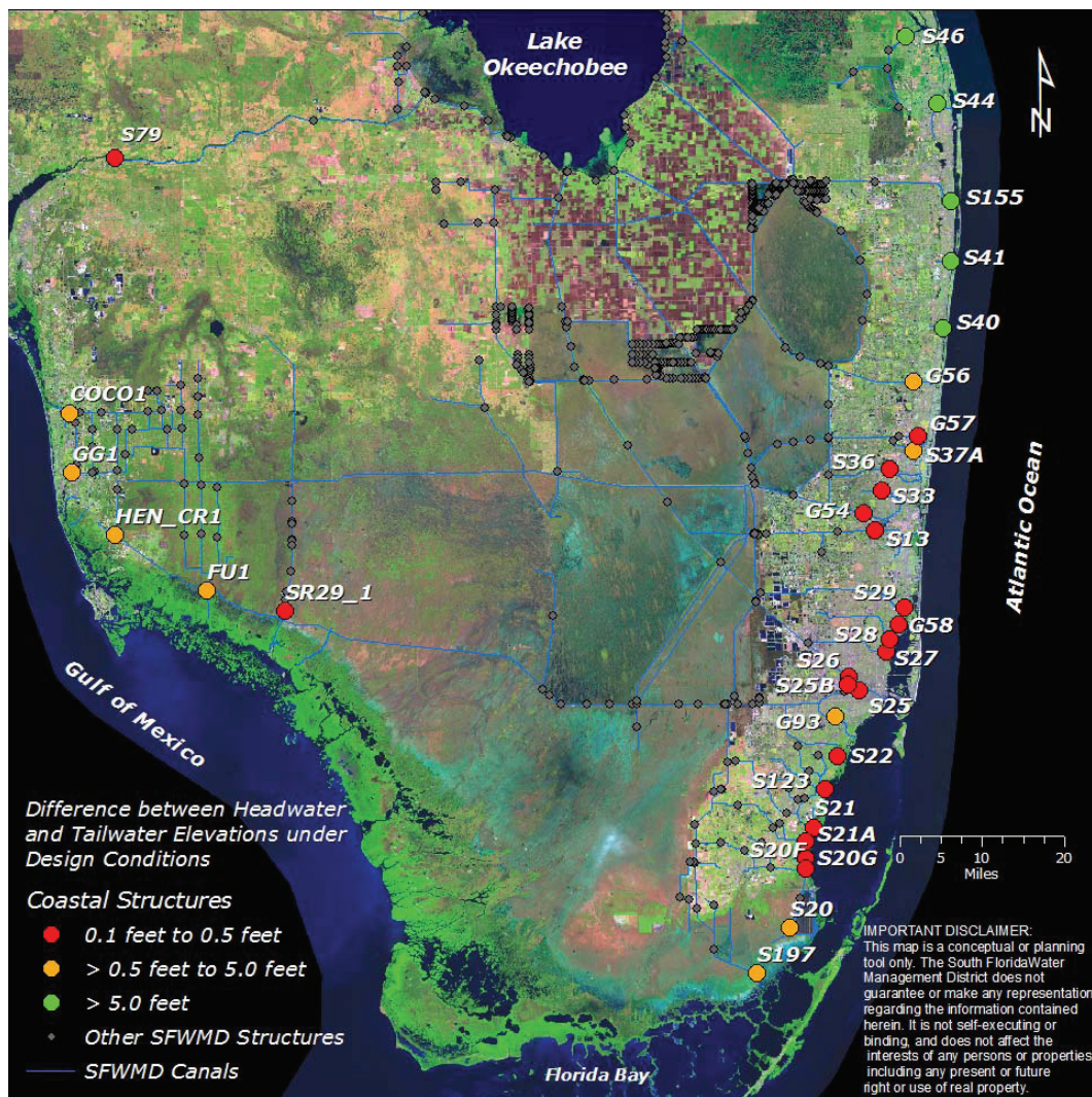
FIGURE 6-6 Vulnerability of coastal structures to potentially rising sea levels. High vulnerability structures are red, medium vulnerability are orange, and low vulnerability are green.
