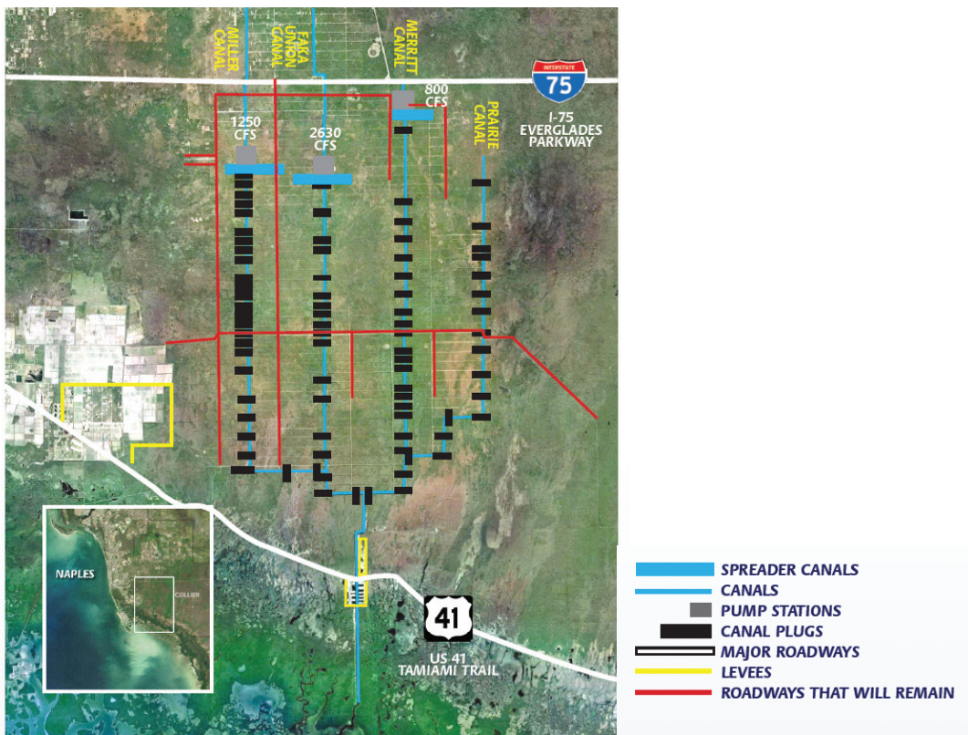
FIGURE 3-2 Components of the Picayune Strand project include road removal, canal plugs, pump stations, spreader canals, and levees.
