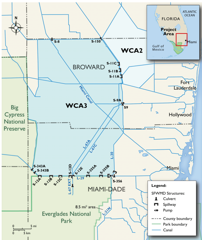
FIGURE 4-6 Water management structures in WCA-3. Gage locations also shown for data presented in Figure 4-7. © International Mapping Associates.
