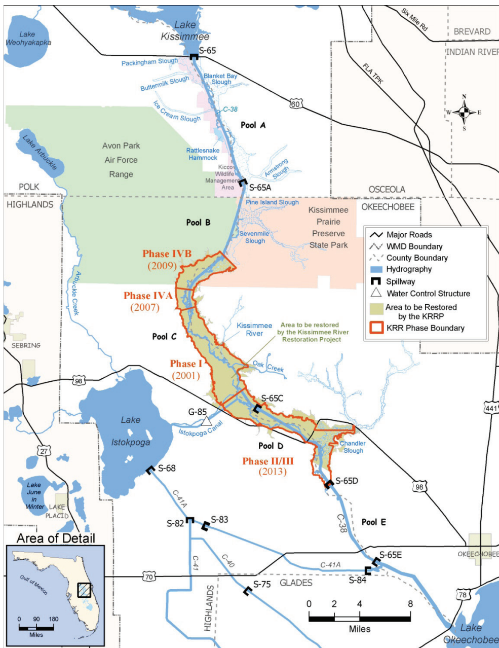
FIGURE 3-11 Phased construction zones in the Kissimmee River Restoration Project.
