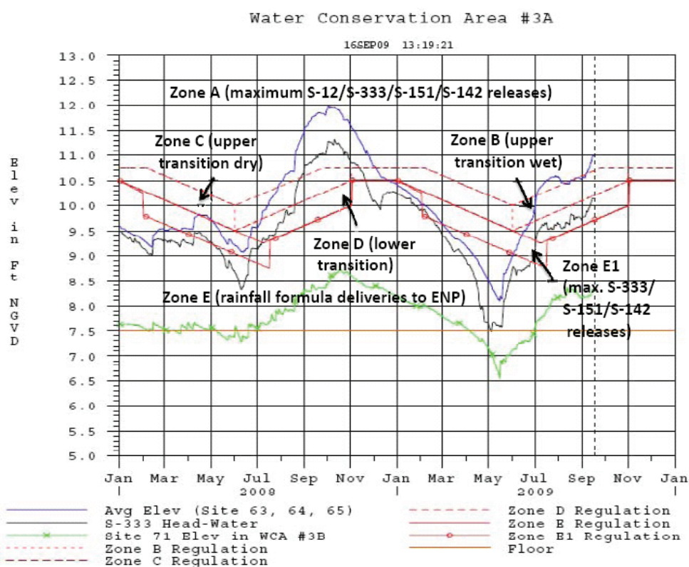
FIGURE D-1 Regulation schedule under the Interim Operational Plan (IOP) for managing water levels in WCA-3A.
