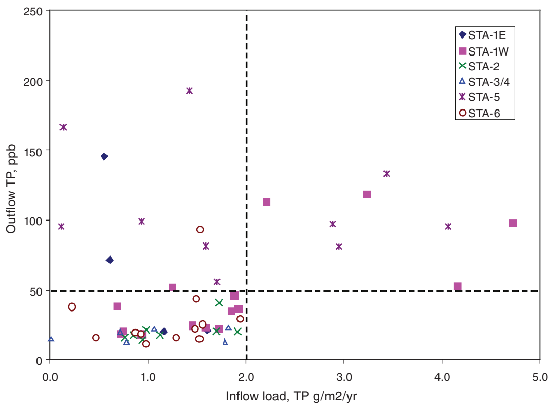
FIGURE 5-10 Relationship between TP inflow load and outflow water column TP concentration of STAs during period of record. Plotted values are mean annual flow-weighted concentrations and mean annual phosphorus loads for each of the STAs over the period of record.
