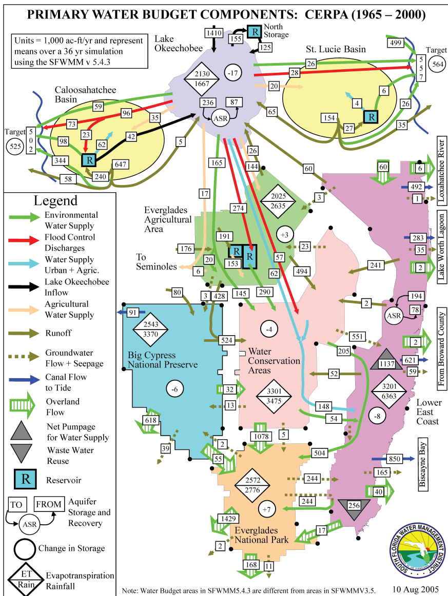
FIGURE 4-5 Estimated annual water budget for the Kissimmee-Okeechobee-Everglades drainage basin under full CERP implementation, calculated using a 36-year simulation using the SFWMM v. 5.4.3. Model run CERP A shown simulates the CERP preferred alternative (D13R). The numbers in rectangles represent mean annual flow volumes in 1,000 acre-feet/year. Change in storage, shown in circles, represents the net inflows minus outflows over the period of record.
