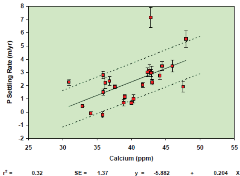
FIGURE 5-17 Relationship of phosphorus settling rate in Lake Okeechobee to calcium concentration in the water column, based on data from 1973 to 1999.
