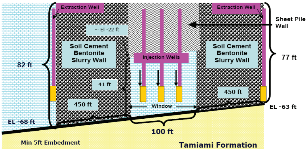
FIGURE 3-7 Schematic diagram of the slurry and sheet pile wall design that will be tested in the L-31N Seepage Management Pilot Project. Placement of injection and extraction wells is also shown.
