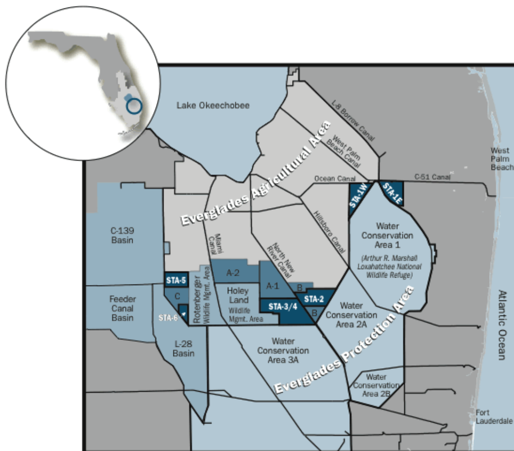
FIGURE 5-6 Location of the six Everglades stormwater treatment areas (STAs): STA-1E, STA-1W, STA-2, STA-3/4, STA-5, and STA-6).
