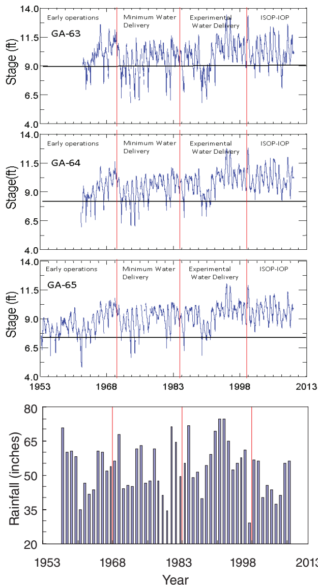
FIGURE 4-7 Water levels at three gauges in WCA-3A: GA-63 at the northern end, GA-64 in the central region, and GA-65 at the southern end. Gage locations shown in Figure 4-6. Major water management regimes are indicated at the top of each hydrograph and average ground elevation by the dark horizontal line. The bottom graph shows annual average rainfall totals across a network of over 50 gages in the NOAA Everglades and southwest coast region, covering the area from Lake Okeechobee southward. Data from the SFWMD and NOAA.
