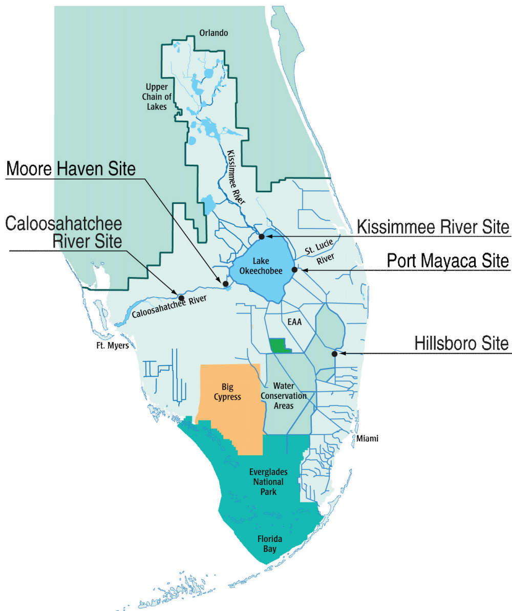
FIGURE 3-6 Locations of the five originally planned CERP ASR pilot projects. Ultimately, pilots were constructed only on the Kissimmee River and the Hillsboro sites because of funding limitations or poor site conditions.
