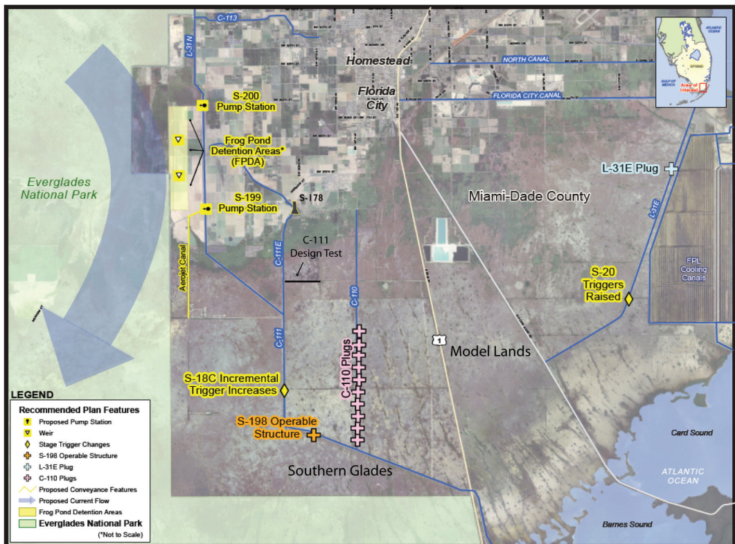
FIGURE 3-4 Features of the western phase of the C-111 Spreader Canal Project.
