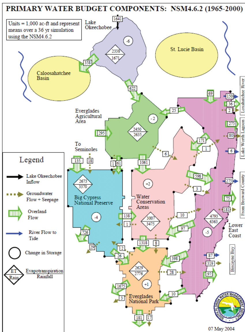
FIGURE 4-1 Estimated annual water budget for the Kissimmee-Okeechobee-Everglades drainage basin, 1965–2000, under pre-drainage and pre-development conditions, calculated using the Natural System Model (NSM) version 4.6.2, which simulates regional hydrology in the absence of existing control structures. The numbers in rectangles represent mean annual flow volumes in 1,000 acre-feet/year, based on model simulations using a 36-year precipitation data set. Change in storage, shown in circles, represents the net inflows minus outflows over the period of record.
