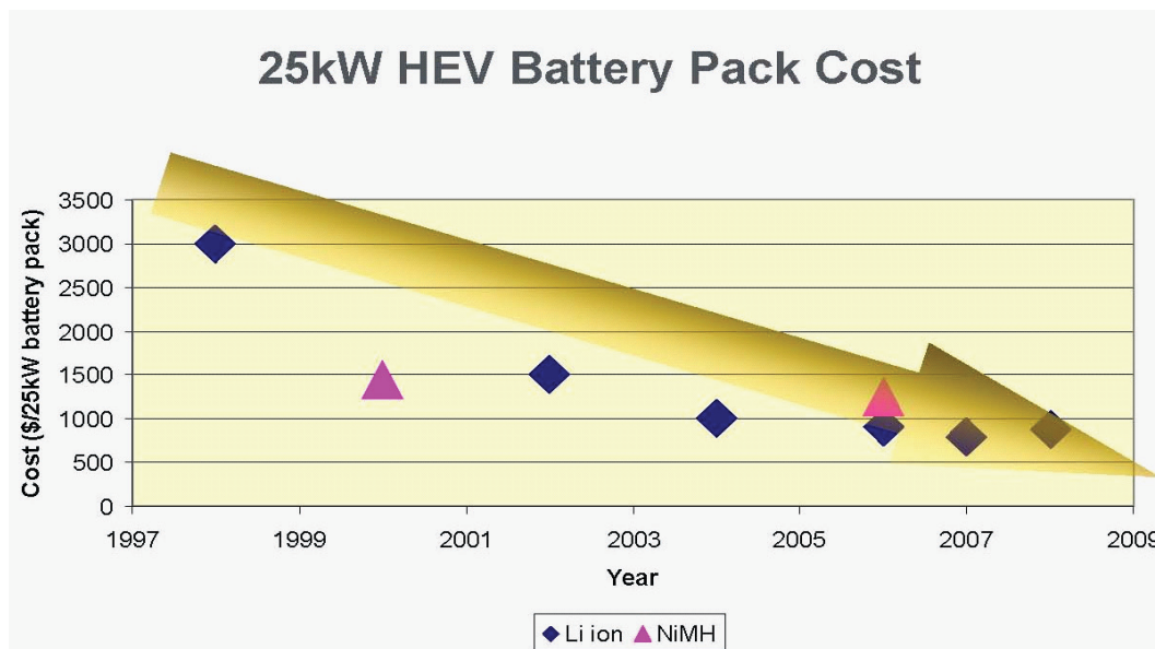
FIGURE F.1 Historical cost reduction experience for NiMH battery packs and for Li-ion battery packs. Recent experience does not suggest rapid further cost reductions. SOURCE: T.Q. Duong, Update on electrochemical energy storage R&D, presentation to the committee, Washington D.C., June 2009.
