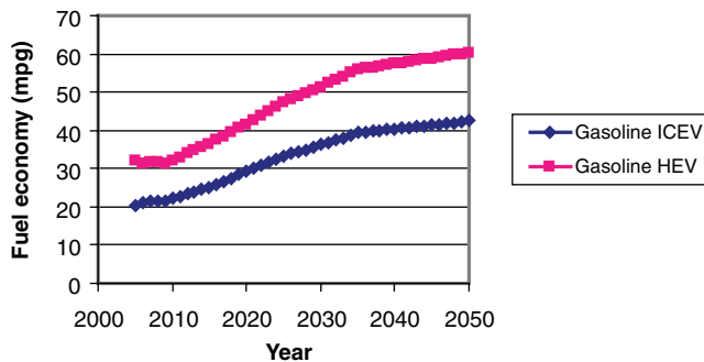
FIGURE C.4 Fuel economy for the ICEV Efficiency Case (Hydrogen Report Case 2). SOURCE: NRC, 2008.
