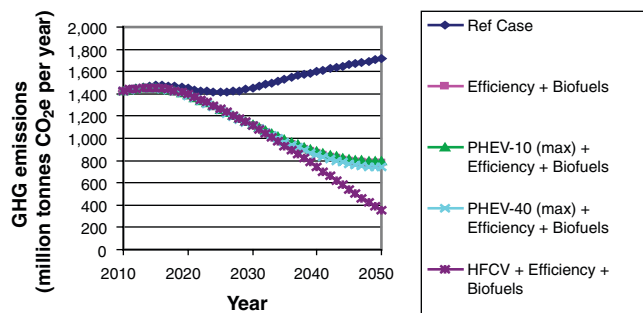
FIGURE 4.20 GHG emissions for scenarios combining ICEV Efficiency Case, Biofuels Case, and PHEVs or HFCVs for the EIA grid mix.
