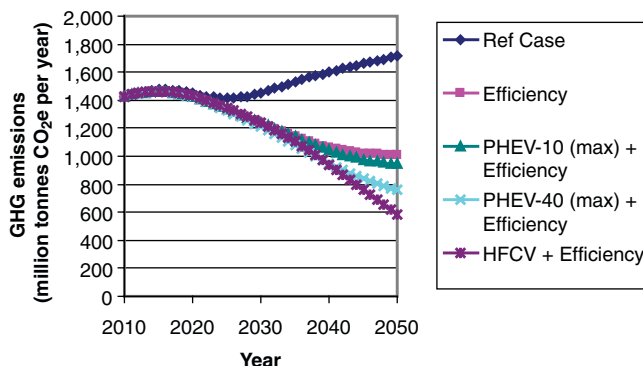
FIGURE 4.19 GHG emissions for cases combining the ICEV Efficiency Case and PHEV or HFCV vehicles for the EPRI/NRDC grid mix.
