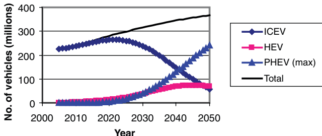
FIGURE C.6 Numbers of light-duty vehicles for portfolio approach, where PHEVs are combined with efficient ICEVs and HEVs.
