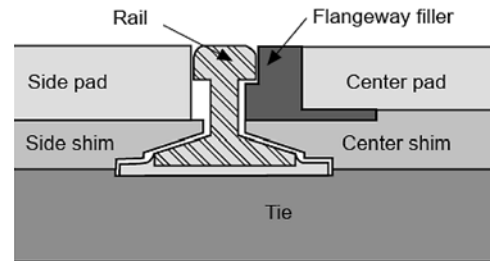
EXHIBIT V-65 Flangeway Filler Strip Applied to the Inside Flangeway (Williams et al., 1998)
