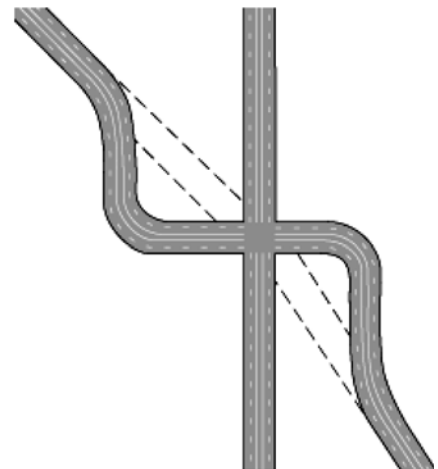
EXHIBIT V-24 Skewed Intersection Realigned to a Right Angle (Oregon DOT, 1995)
