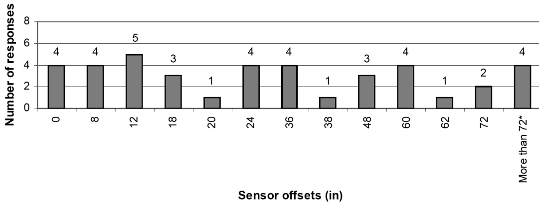
FWD Sensor Spacings Used by State Highway Agencies on Rigid Pavements at the Network Level
