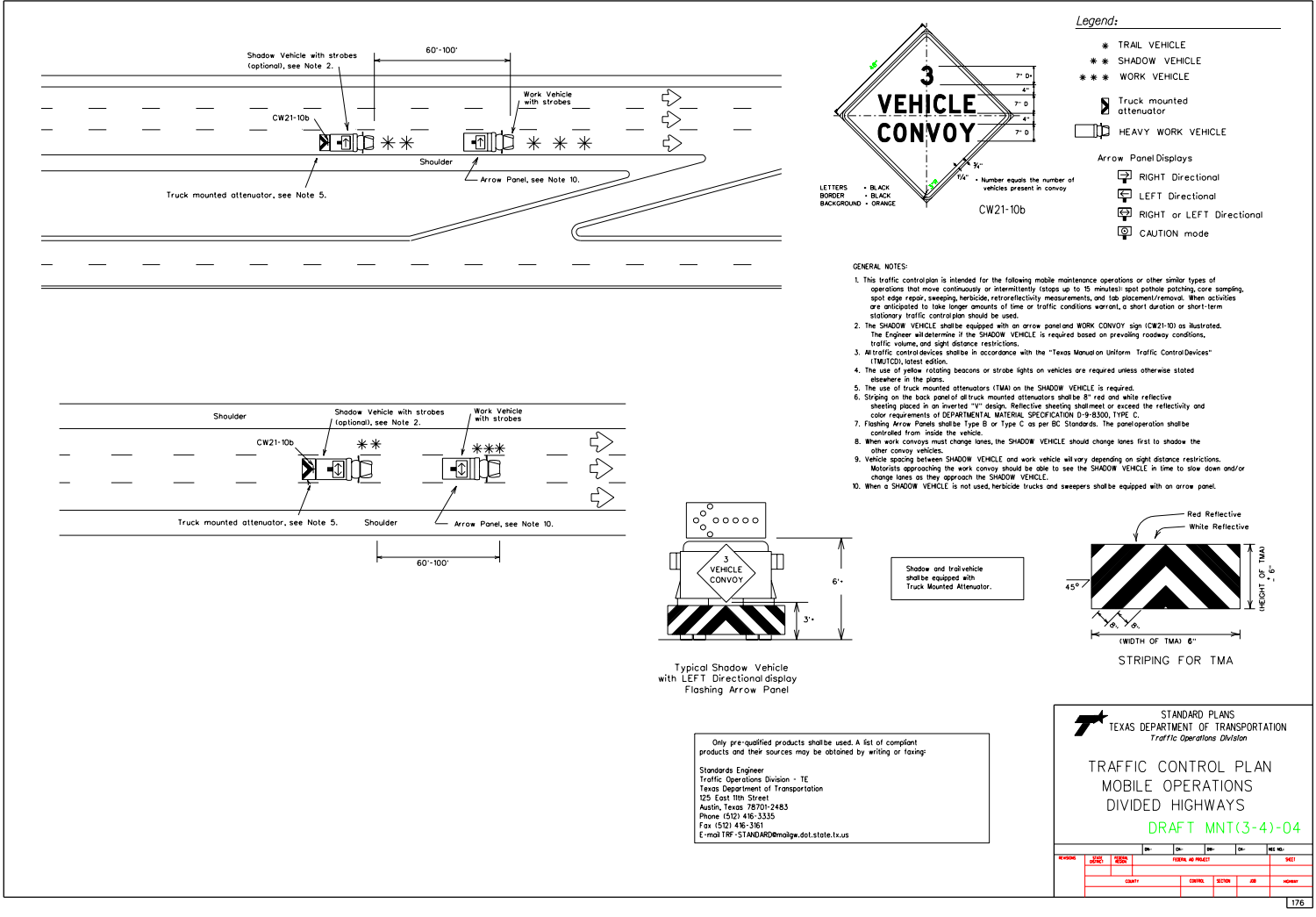
FIGURE 4 Mobile maintenance traffic control plan for spot pothole patching, spot edge repair, sweeping, herbicide, retroreflectivity measurements, core sampling, tab placement–removal, and other similar operations on divided highways.
