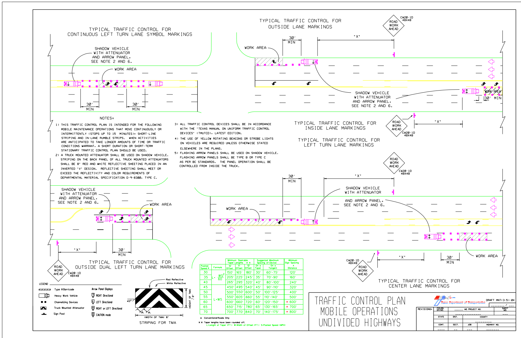
FIGURE 5 Mobile maintenance traffic control plan for short-line striping and in-lane (lateral) rumble strips on undivided highways.
