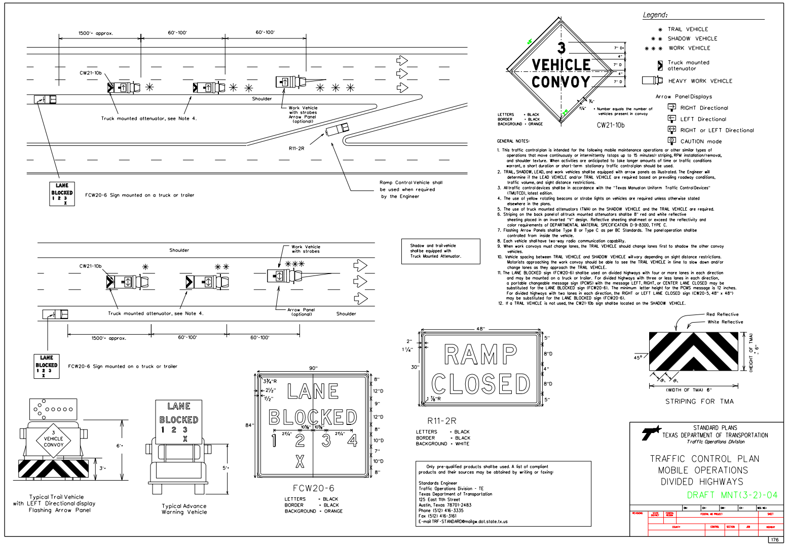
FIGURE 2 Mobile maintenance traffic control plan for striping, RPM installation-removal, shoulder texture, and other similar operations on divided highways.
