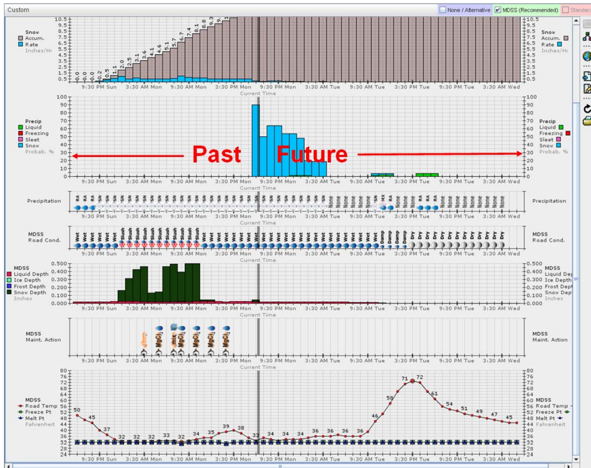
FIGURE 6 The PF MDSS forecast treatment recommendation screen. Like the prototype MDSS display, the PF version provides advanced visualization graphics on precipitation type and accumulation, road temperature forecasts, and treatment recommendations specifically tailored for winter maintenance personnel.
