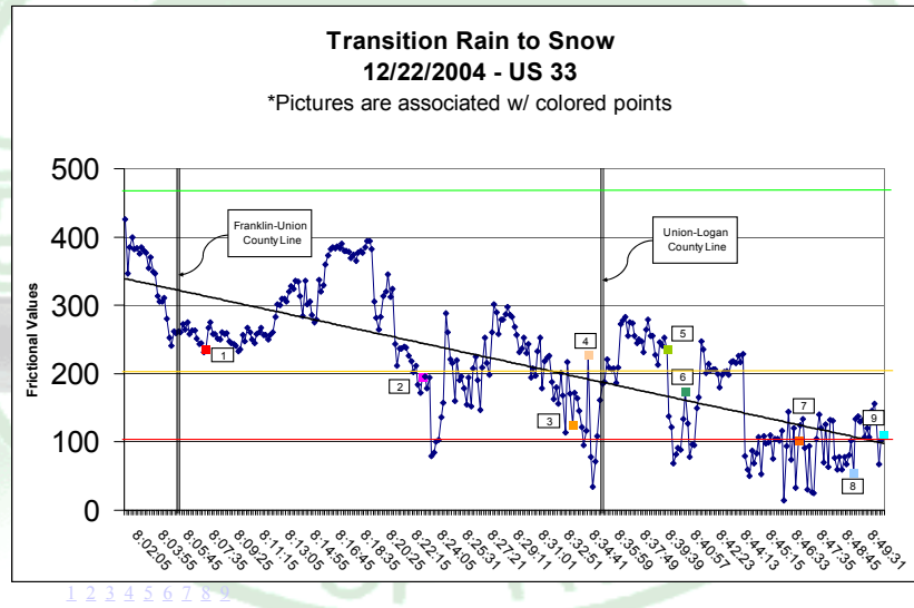
FIGURE 6 Transition graph.
