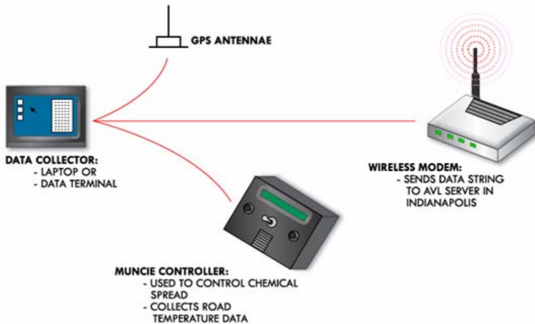
FIGURE 3 Vehicle hardware.
