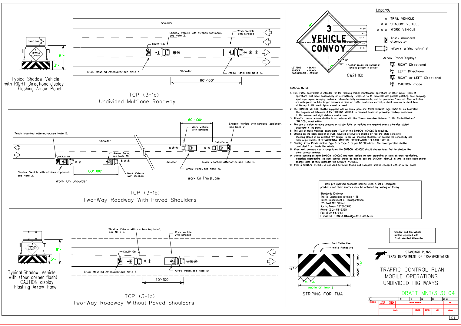
FIGURE 3 Mobile maintenance traffic control plan for spot pothole patching, spot edge repair, sweeping, herbicide, retroreflectivity measurements, core sampling, tab placement–removal, and other similar operations on undivided highways.
