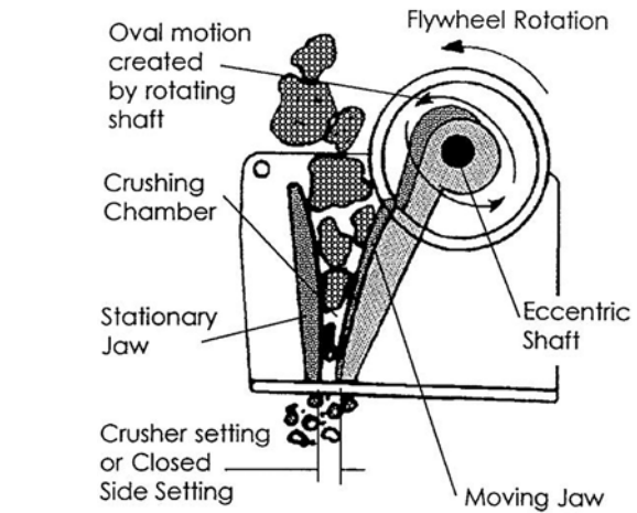
Figure 19. Schematic of a jaw-type crusher (156).
