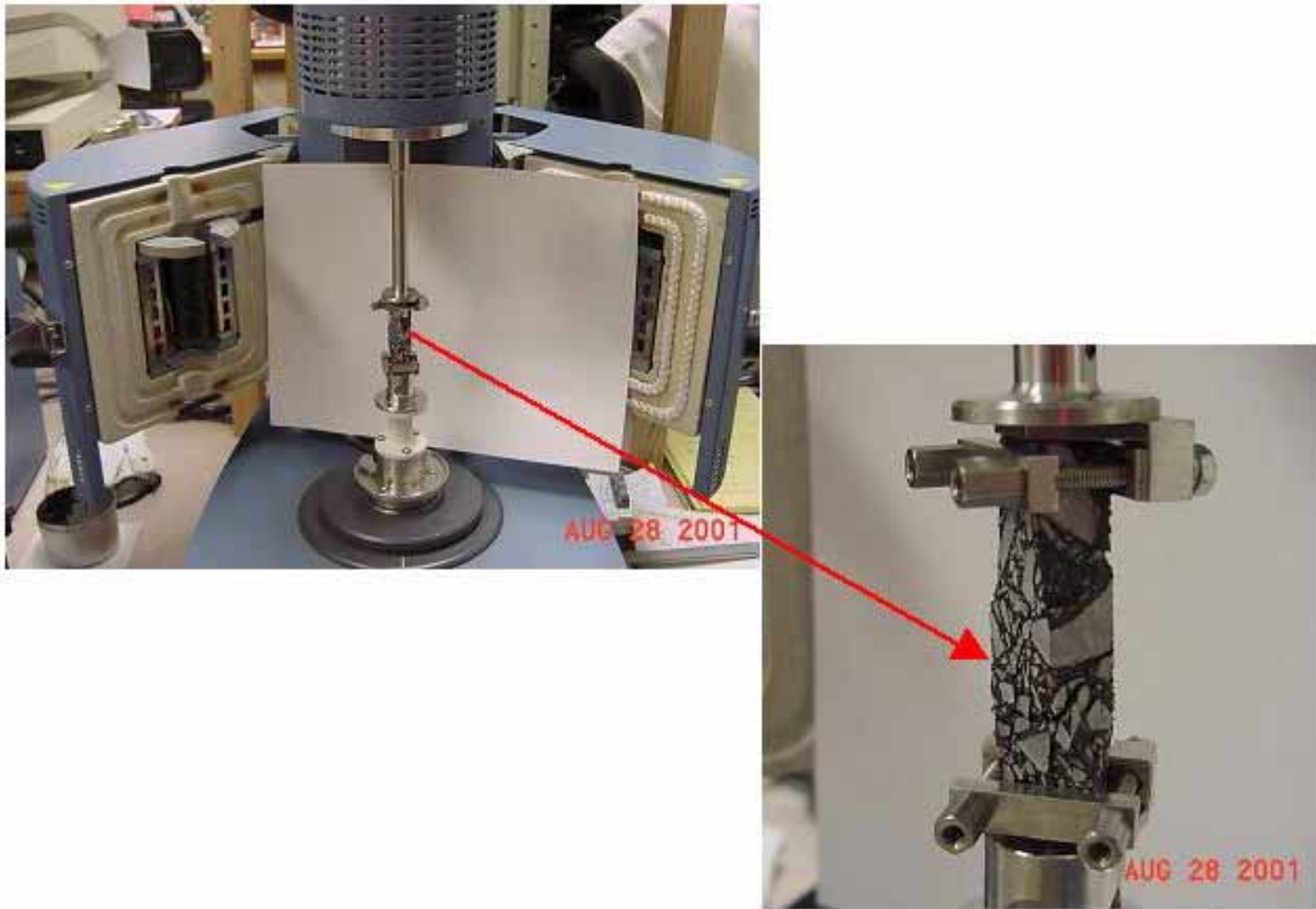
FIGURE 7 Typical test specimen mounted in rheometer and close-up showing specimen after testing.
