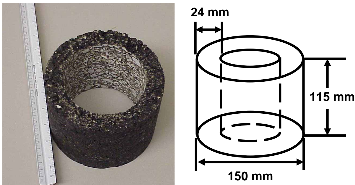
FIGURE 1 Hollow cylinder specimen and typical dimensions.
