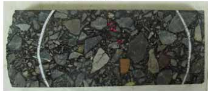
FIGURES 1 through 4 Initial steps in cutting gyratory pill to obtain test specimens.
