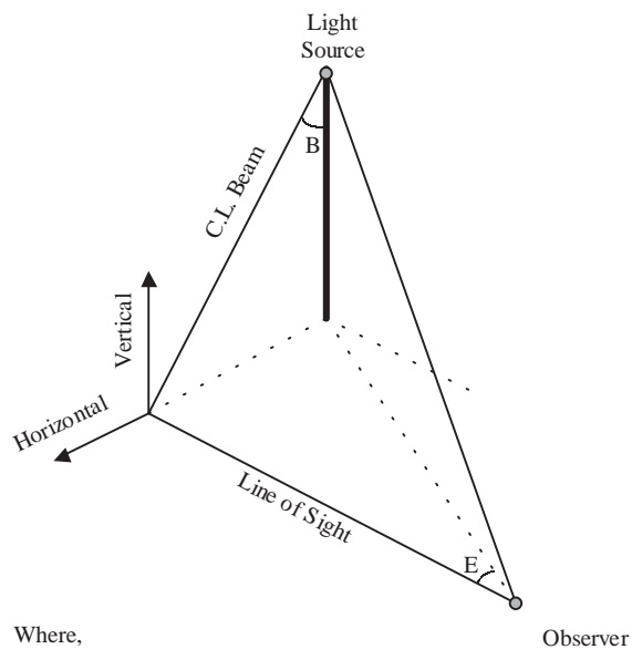
Figure 5. Effect of beam angle and eccentricity in reducing glare.
