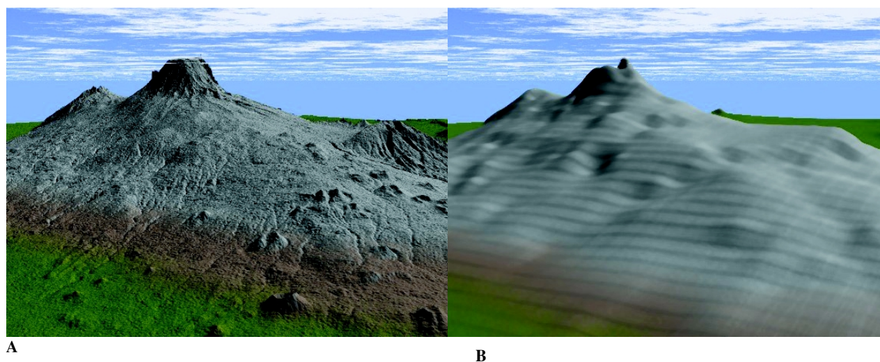
FIGURE 5-9 (a) SRTM 30 \times 30 m digital elevation model of Mount Kilimanjaro in Tanzania and Kenya observed from an oblique vantage point looking W-NW. Note the detail associated with the small cinder cones on the flank of the mountain. (b) GTOPO30 1 \times 1 km data of the same region (NASA Jet Propulsion Laboratory and U.S. Geological Survey EROS Data Center). The distance between the two peaks is 70 km.
