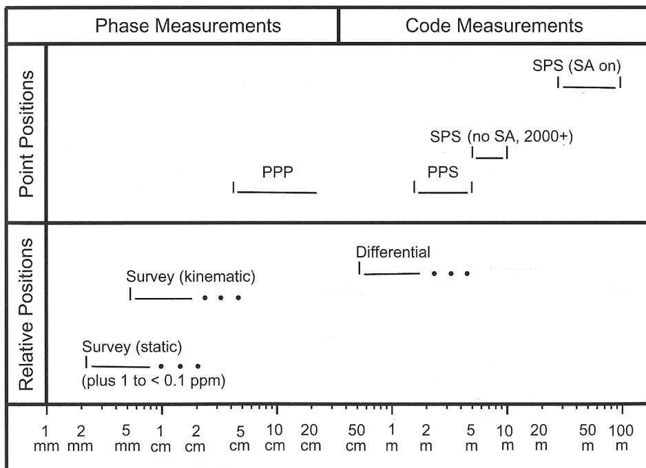
FIGURE 5-A1 Global Positioning System accuracy and positioning modes (adapted from Rizos [2002]). The top half of the illustration refers to single point positioning measurements made with a single GPS unit communicating with a number of satellites. The lower half refers to the relative positioning mode where the position of the receiver of interest (i.e., the location of the user) is derived relative to a base station receiver with known absolute coordinates.
