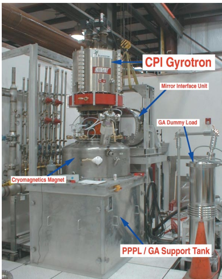
FIGURE 2.2 A gyrotron from the DIII-D tokamak experiment at General Atomics (GA) in San Diego. A gyrotron is a source of high-frequency radio waves for heating electrons. Courtesy of General Atomics.
