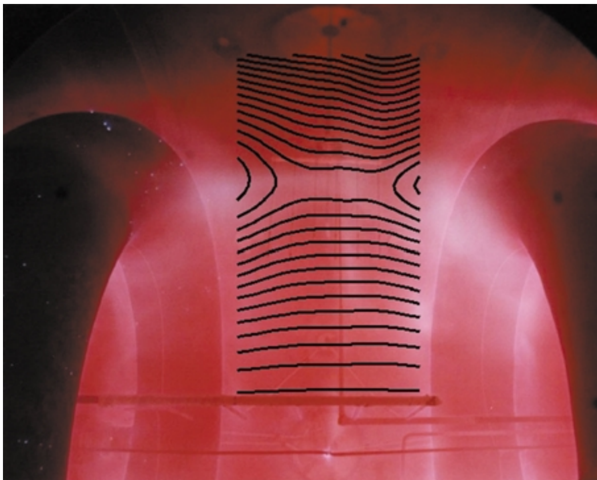
FIGURE 4.4 This image shows the interior of the MRX reconnection experiment. The pair of large coils produce oppositely directed magnetic field lines. The bright area between the coils (in an X-shaped pattern) is the region where magnetic energy is being released into the plasma through the reconnection process. Superimposed is a snapshot of the measured magnetic field. Courtesy of M. Yamada (PPPL). Reprinted by permission from Journal of Geophysical Research , 1999, vol. 104, p. 14529.
