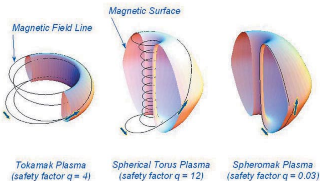
FIGURE 3.2 Examples of the magnetic topologies of several related toroidal configurations with increasing curvature and varying stability characteristics. The tokamak (left) uses a strong external toroidal field to provide robust stability against pressure- and current-driven instabilities. The spherical torus uses a weak toroidal field in a compact configuration to allow access to higher \beta values than obtained in the tokamak. The spheromak (right) uses internal plasma currents only to provide the confining poloidal field plus a weak toroidal field. A larger safety factor indicates a higher level of protection from current-driven instabilities. Courtesy of M. Peng (PPPL). Reprinted by permission from Physics of Plasmas , 2000, vol. 7, pp. 1681-1692.
