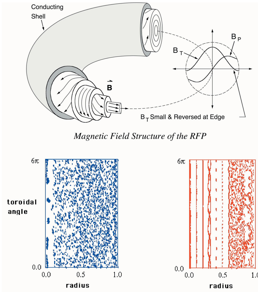
FIGURE 3.3 A magnetic confinement concept such as the reversed-field pinch (top) is a relatively self-organizing configuration that is subject to turbulent magnetic field structures. The magnetic topology includes a reversal of the toroidal field inside the plasma owing to plasma currents. Under normal inductive current drive, the magnetic field lines can readily become chaotic, as indicated by a puncture plot of the field lines as they traverse a poloidal plane (bottom left). With finer control of the plasma currents, well-defined flux surfaces are restored (bottom right). Courtesy of S. Prager (University of Wisconsin at Madison).
