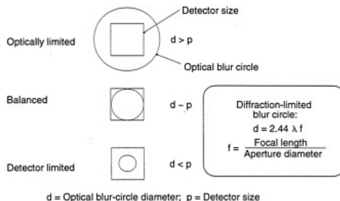
Figure 3.5 Different design approaches yield a 4:1 range in aperture size (or equivalently in focal ratio).
