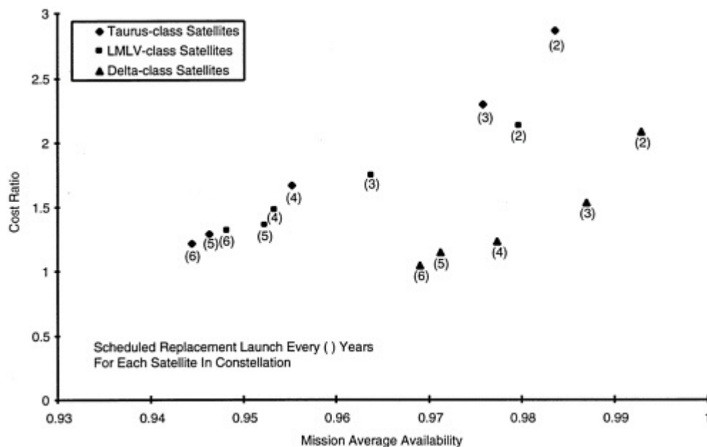
Figure 6.2 Mission cost sensitivity to average availability: operational mission model.
