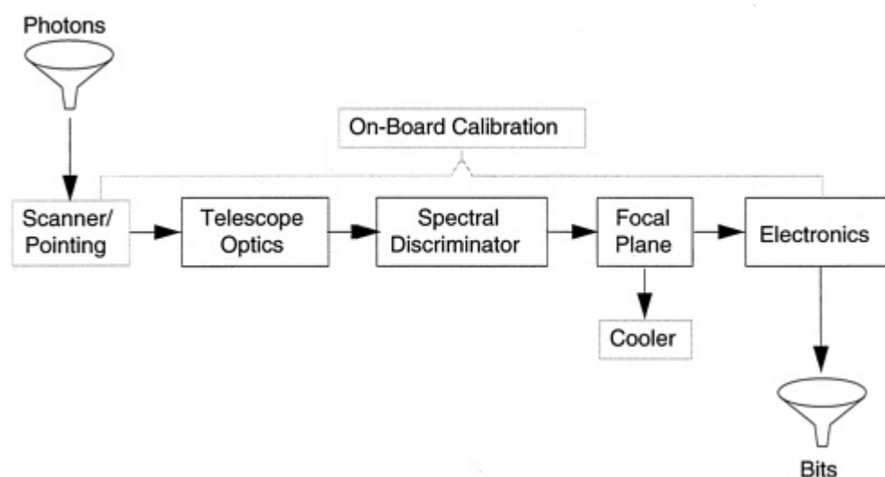
Figure B.1 Depiction of the generic electro-optical sensor.
