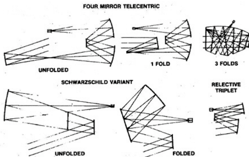
Figure B.2 This scale drawing of different telescope designs, all with the same aperture diameter and focal length, shows striking differences in packaging efficiency. Reflective triplet is most compact.
