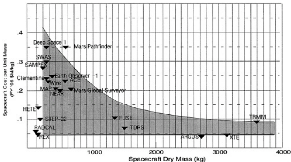
Figure 4.1 The relative cost of small spacecraft (adapted from Sarsfield, 1997). Note that all acronyms are defined in Appendix E .
