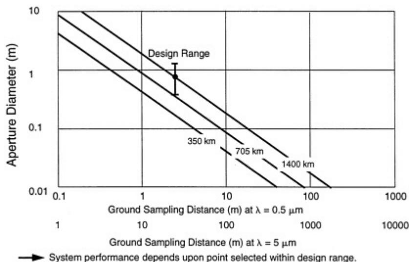
Figure 3.4 Diffraction dictates aperture size.
