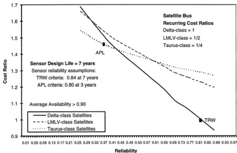
Figure 6.1 Relationship between mission cost and sensor reliability: operational mission model.
