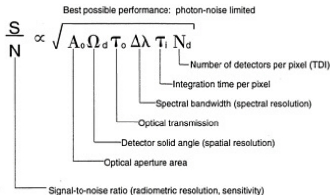
Figure 3.3 Factors determining detector signal-to-noise ratio.
