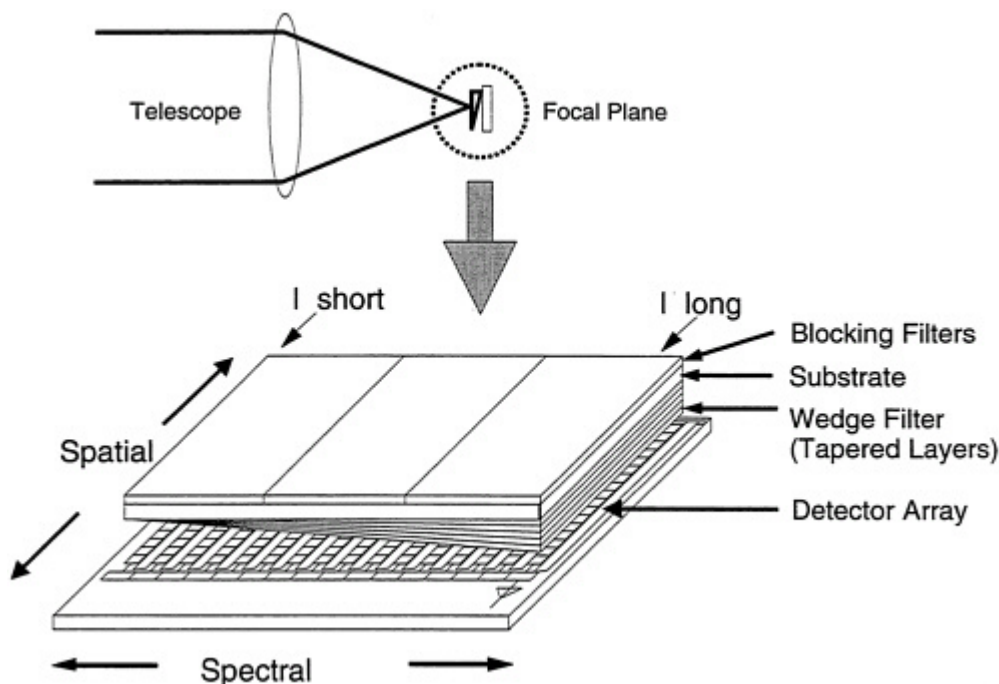
Figure B.4 Wedge spectrometer approach reduces size and mass of hyperspectral sensors.
