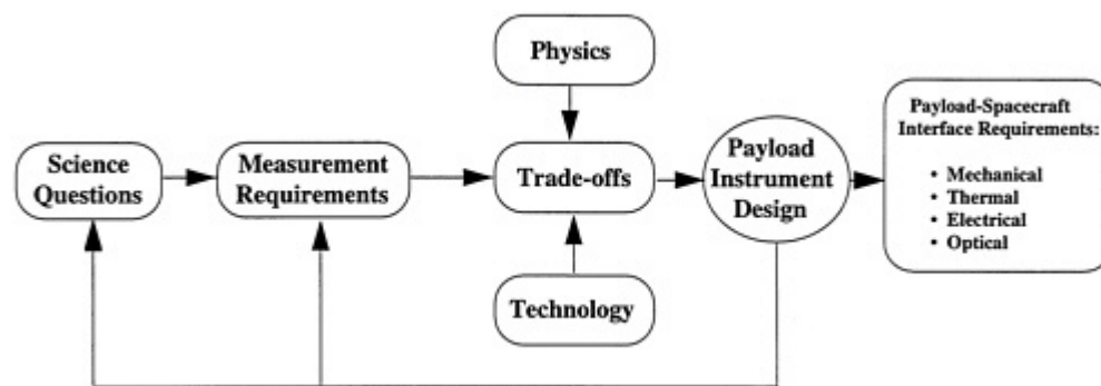
Figure 3.1 The payload design process generates requirements for accommodating the payload.
