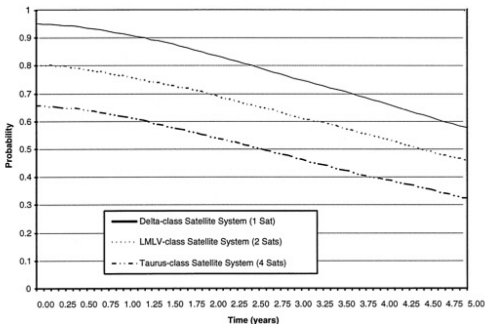
Figure 6.4 Probability of operation with no failures versus time: science mission model.
