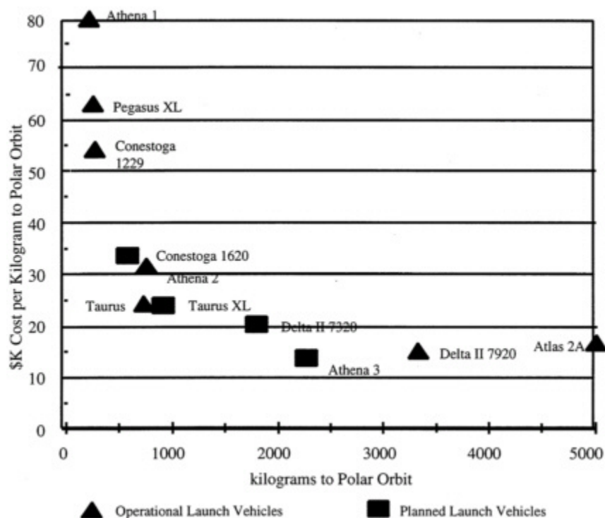
Figure 5.1 Launch vehicle cost per unit mass to EOS orbit.
