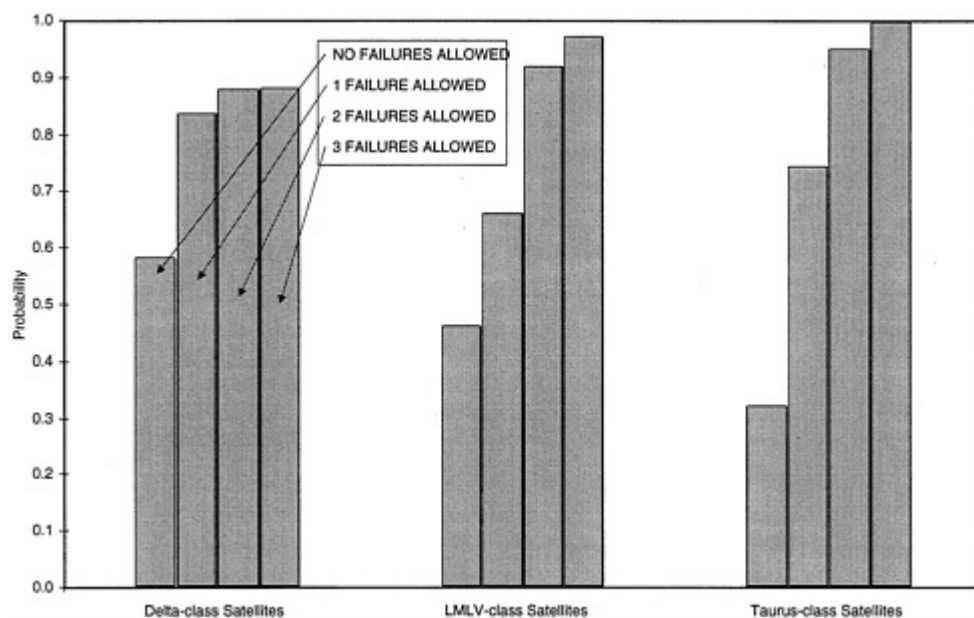
Figure 6.5 Probability of mission success defined in terms of a specific number of failures: science mission model.
