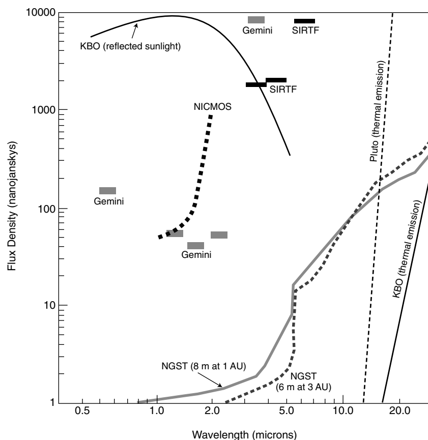
FIGURE 4.1 The estimated sensitivities of various ground- and space-based facilities likely to play roles in studies of trans-neptunian objects in the next 10 to 15 years. The current capabilities of the Hubble Space Telescope's Near Infrared Camera and Multi-Object Spectrometer (NICMOS) are plotted relative to those of the 8-meter Gemini telescope currently under construction in Hawaii, and the Space Infrared Telescope Facility scheduled for launch in 2001. Also shown are two different concepts for NASA's proposed Next Generation Space Telescope (NGST). The 6-meter NGST is in a heliocentric orbit at 3 AU, i.e., in the outer portion of the asteroid belt where the zodiacal emission is 30 to 100 times lower than it is at 1 AU. The 8-meter NGST is in a heliocentric orbit at 1 AU. Gemini (outfitted with low-order adaptive optics), NICMOS, SIRTf, and NGST will readily detect the reflected sunlight from Pluto (off scale) and a typical KBO out to wavelengths of \sim 5 microns. Pluto's thermal emission should be detectable by either of the two NGST concepts at wavelengths greater than \sim 15 microns. The thermal emission from the KBO, however, appears to be beyond the capability of any of the facilities in the wavelength range illustrated. SIRTf will, however, be able to detect such a KBO at wavelengths greater than 35 microns (not illustrated). The capabilities indicated assume a 10,000-sec integration, a 10\text{-}\sigma signal-to-noise ratio, and a wide bandpass of \lambda/\Delta\lambda = 3 . The Kuiper Belt object is taken to have a radius of 100 km and is located at 35 AU. Its temperature is 35 Kelvin; it has a visual magnitude of 22.0 and a V\text{-}K color index of 2.0 (i.e., the red color characteristic of some, but not all, trans-neptunian objects). Pluto is assumed to have a diameter of 1,200 km and a temperature of 40 Kelvin, and to be located at its current distance from the Sun. Adapted from The Next Generation Space Telescope: Visiting a Time When Galaxies Were Young , H.S. Stockman, ed., Space Telescope Science Institute, Baltimore, Maryland, 1997, with information on Pluto and the KBO courtesy of D.P. Cruikshank.
