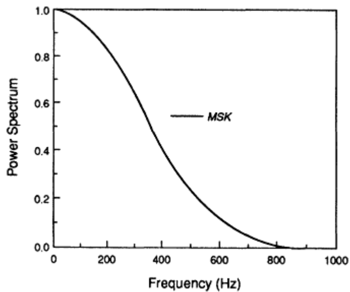
Figure 2-2. Minimum shift keying (MSK), 1,200 bits/sec.
