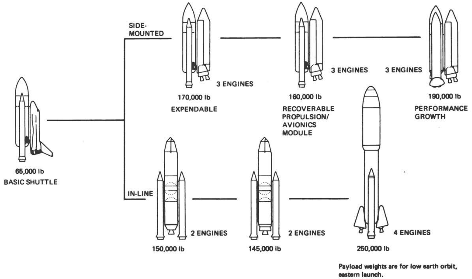
Figure 7 Potential Heavy Lift Vehicles (U.S. Air Force)
