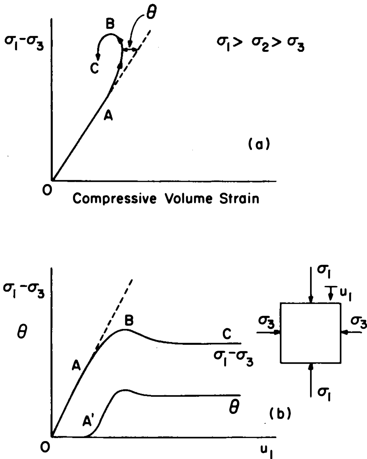
FIGURE 3 Signatures of microcrack accumulation and evolution of a nucleus of a shear fault: (a) dependence of compressive volumetric strain on net compressive stress ( \sigma_1 - \sigma_3 ), showing the increased inelastic dilatation due to microcracking along path AB and the unloading upon faulting along path BC and (b) dependence of net compressive stress ( \sigma_1 - \sigma_3 ) and dilatation \theta on compressive displacement u_1 .
