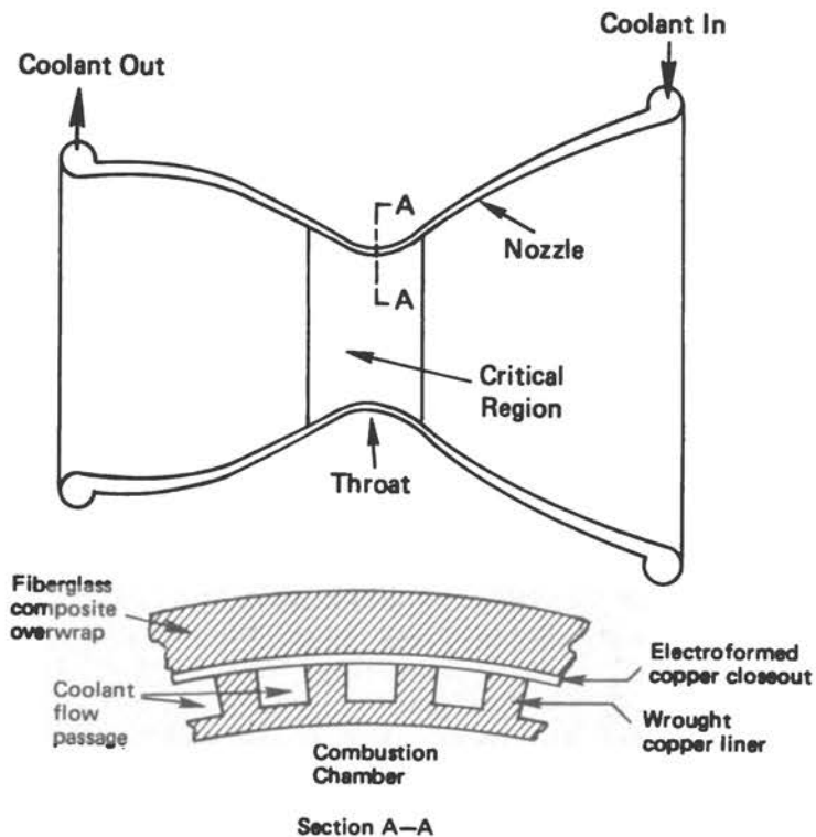
FIGURE 15 Regeneratively Cooled Low-Stiffness Thrust Chamber Closeout
