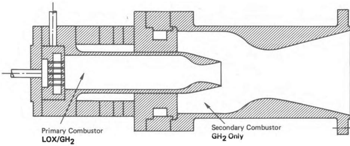
Dual Throat Combustor
